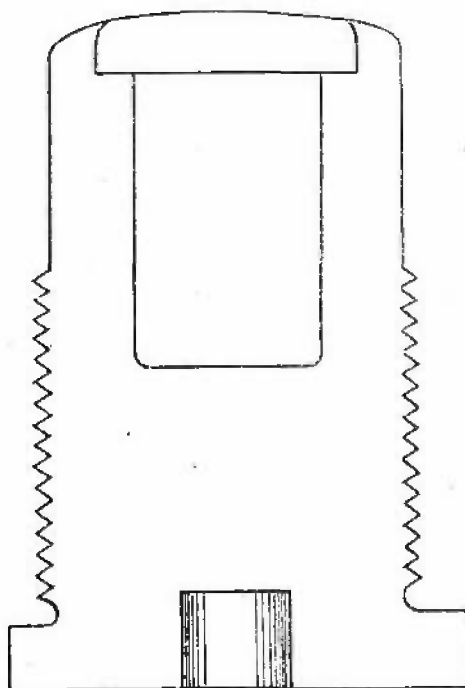
PLUG, BASE, SHELL, NO. 2, MARKS I to IV.
