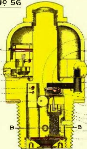
SECTION AT A A.
