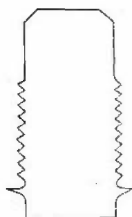
Fig. 68. PLUG, BASE, SHELL, NO. 3.
