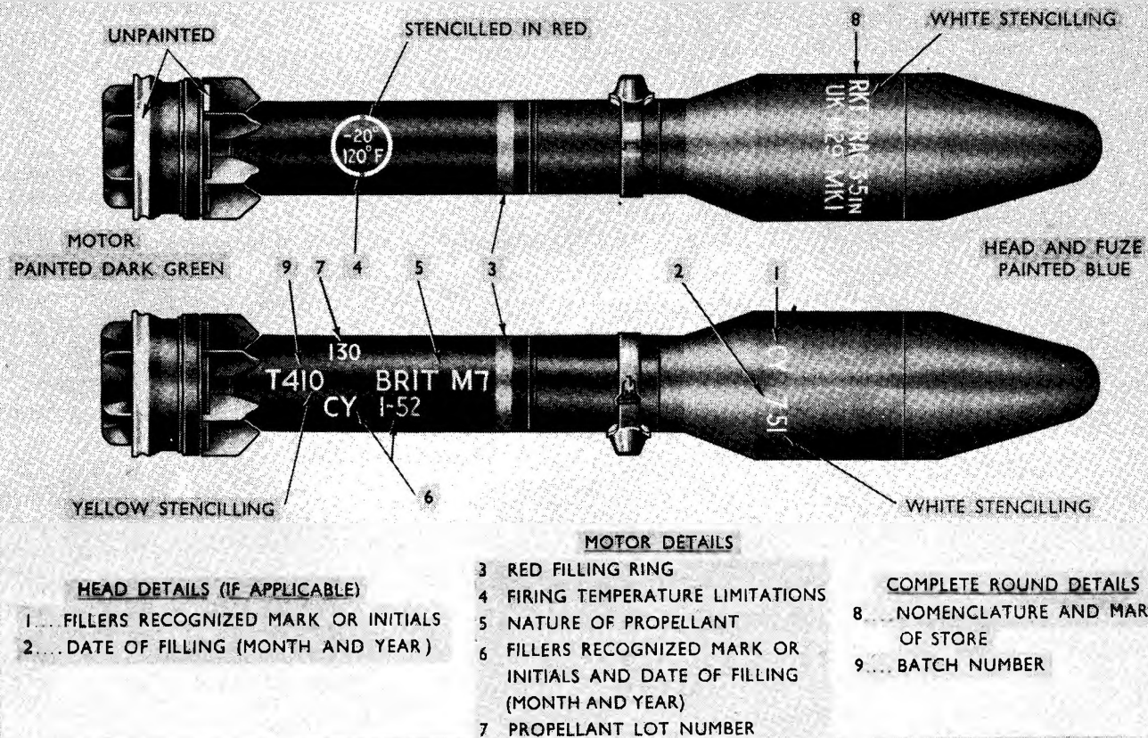
Fig. 32 Painting and Stencilling Practice Rocket (U.K. Manufacture)
