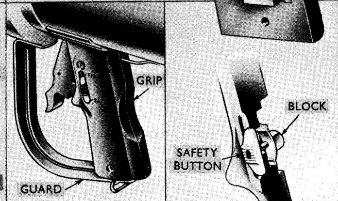
Fig. 8 Firing Mechanism
