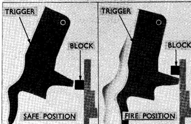
Fig. 8 Firing Mechanism
