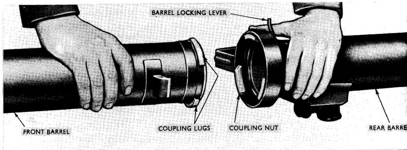
Fig. 1 Assembling of Barrel
