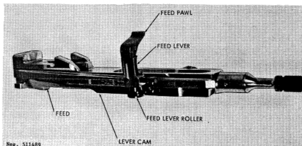
Figure 190. Vz59 feed device.
