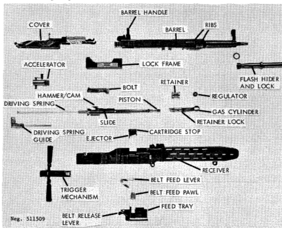
Figure 210. ZB-37 disassembled.
