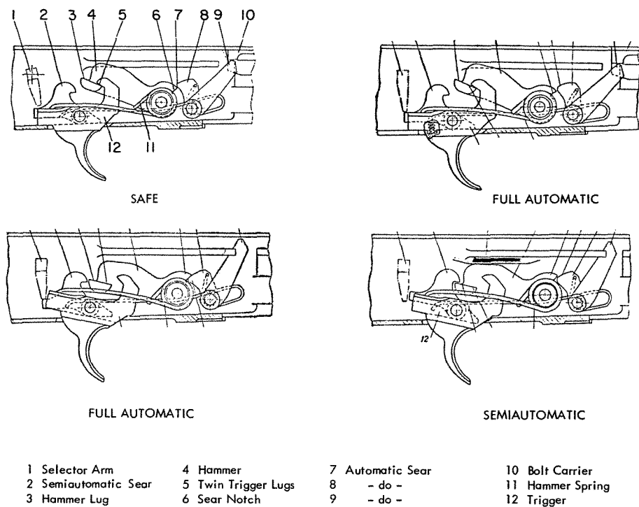
Figure 70. AK-47 trigger mechanism.
