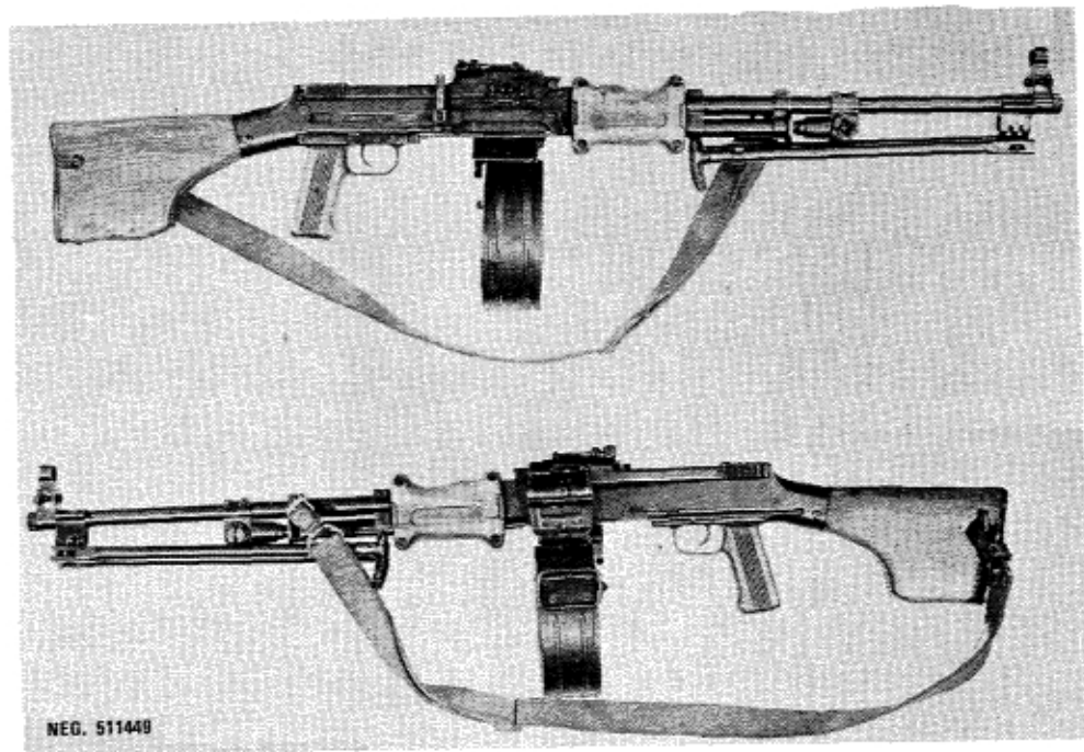
Figure 150. PRC Type 56 light machinegun.
