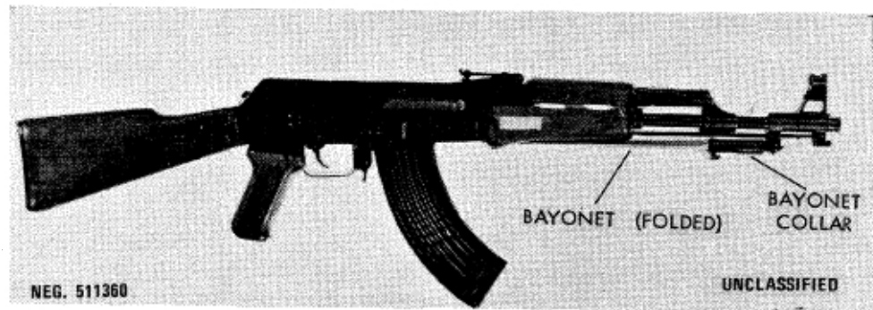
Figure 61. Late model PRC Type 56 assault rifle.
