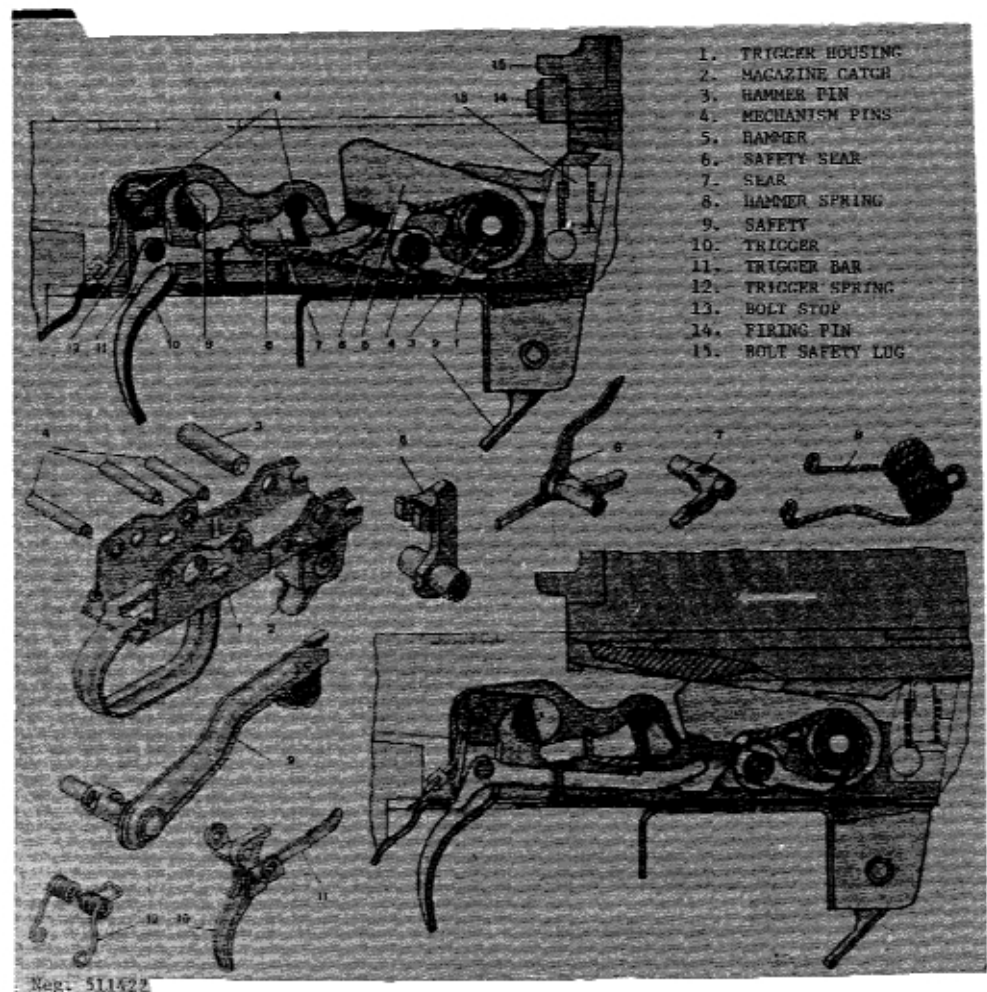
Figure 123. SVD trigger mechanism section.
