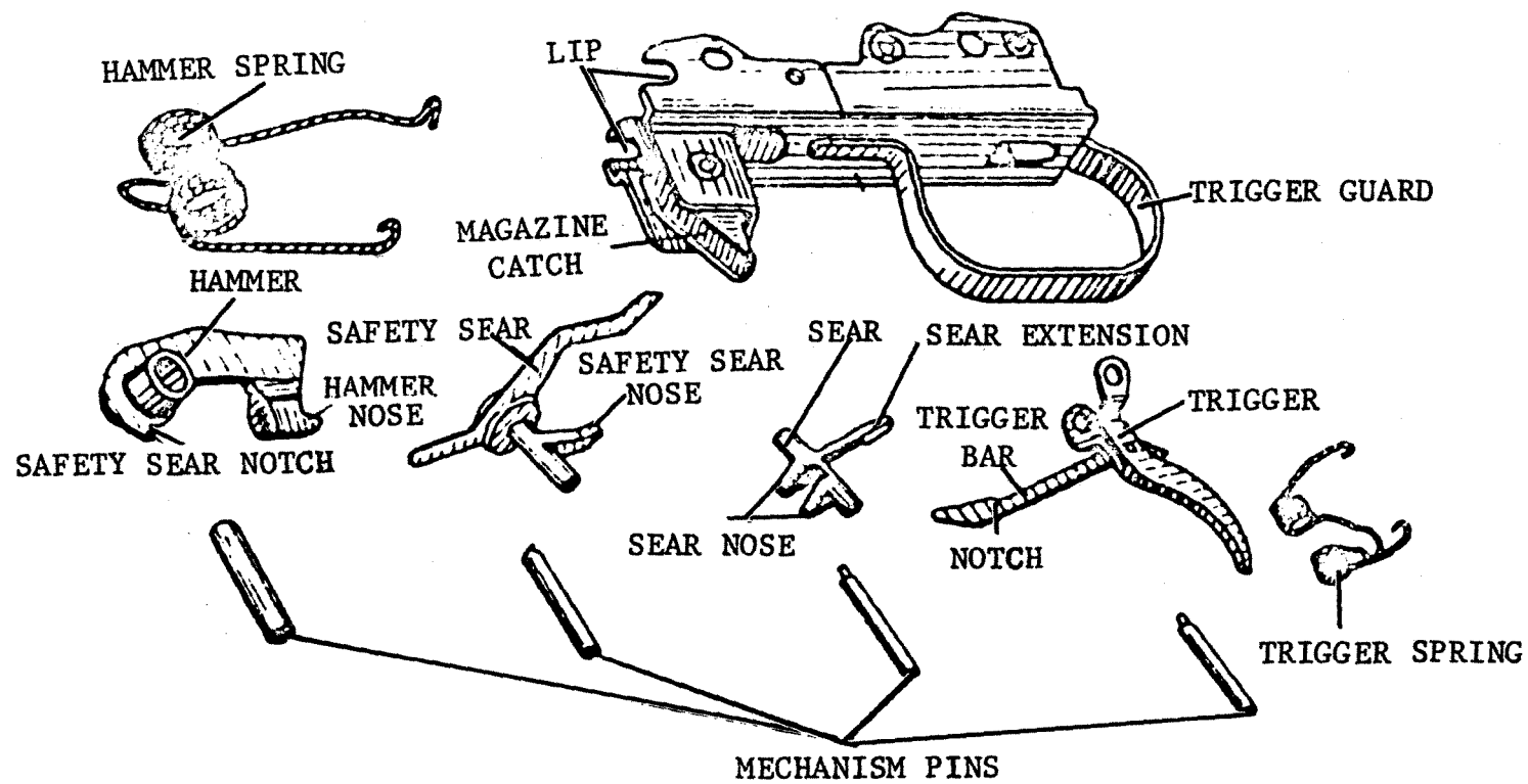
Figure 122. SVD trigger mechanism parts.
