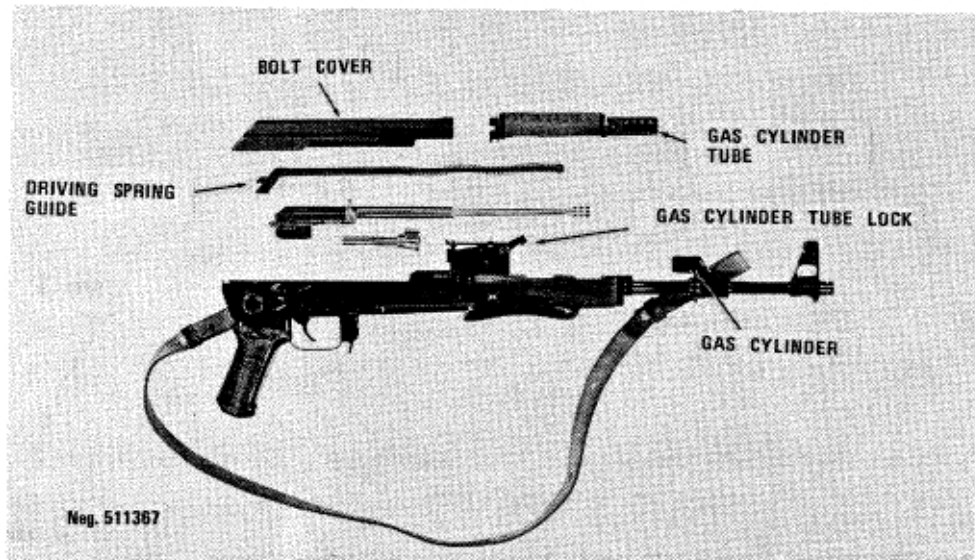
Figure 68. AK-47 field stripped.
