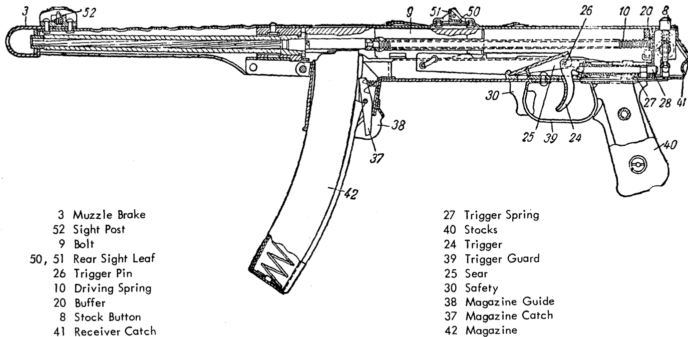
Figure 41. PPS-43 section.
