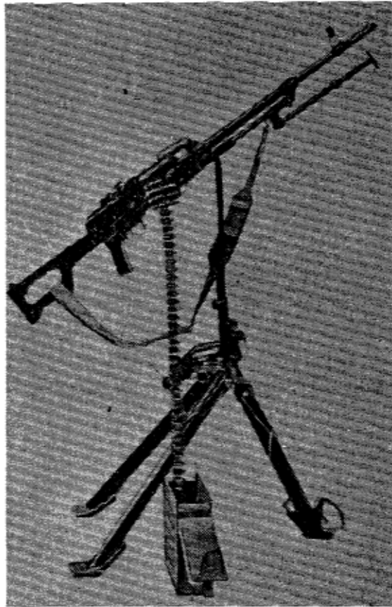
Figure 182. PKM set up for antiaircraft fire.
