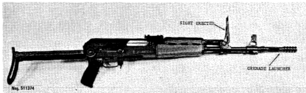
Figure 75. Yugoslav grenade launcher.
