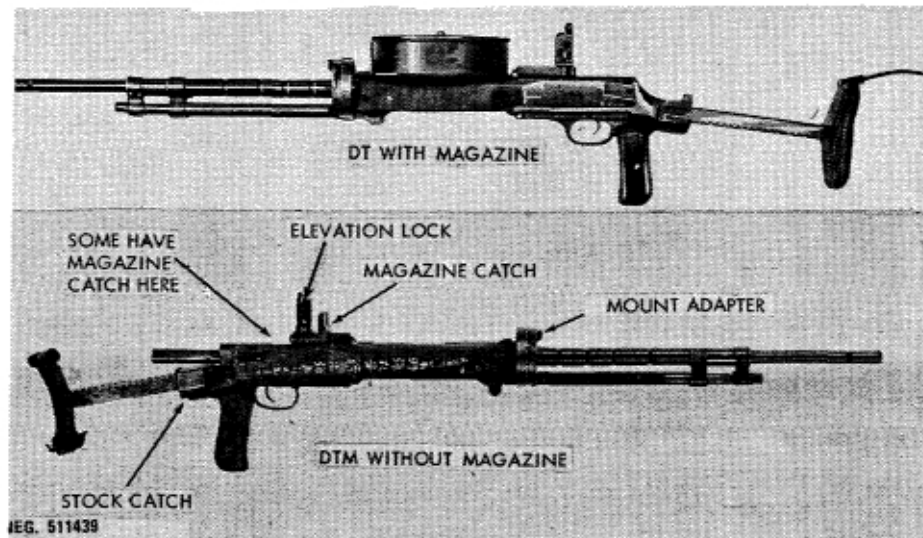
Figure 140. DT and DTM tank machinegun.
