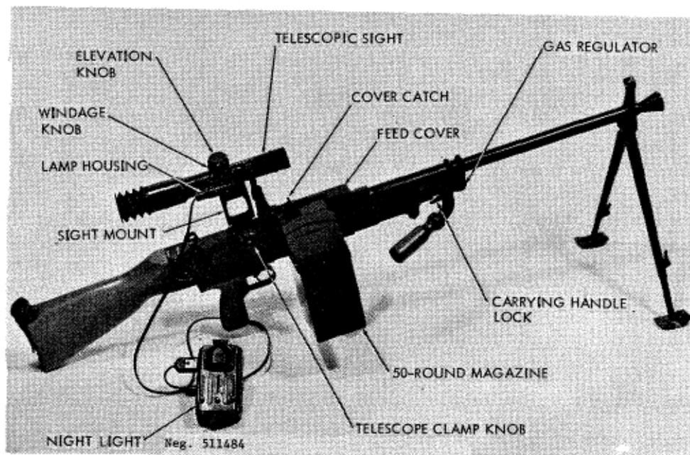
Figure 185. Vz59L squad light machinegun with telescope sight.
