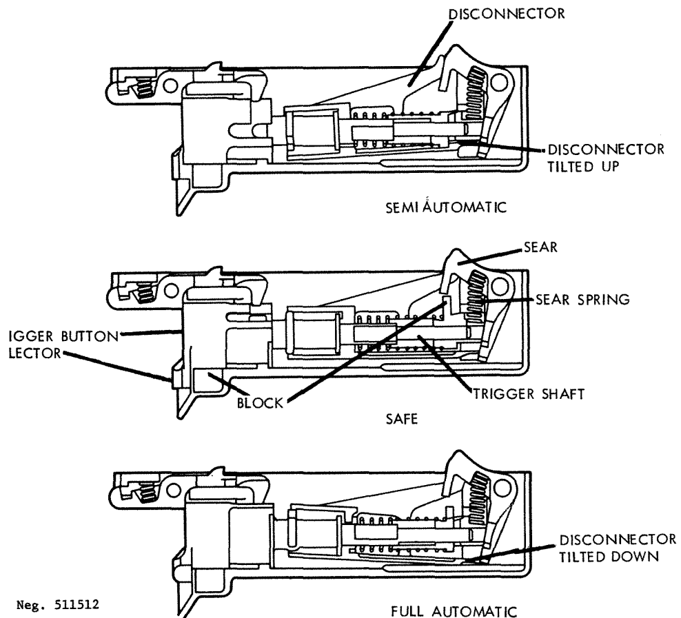
Figure 213. ZB-37 trigger mechanism.
