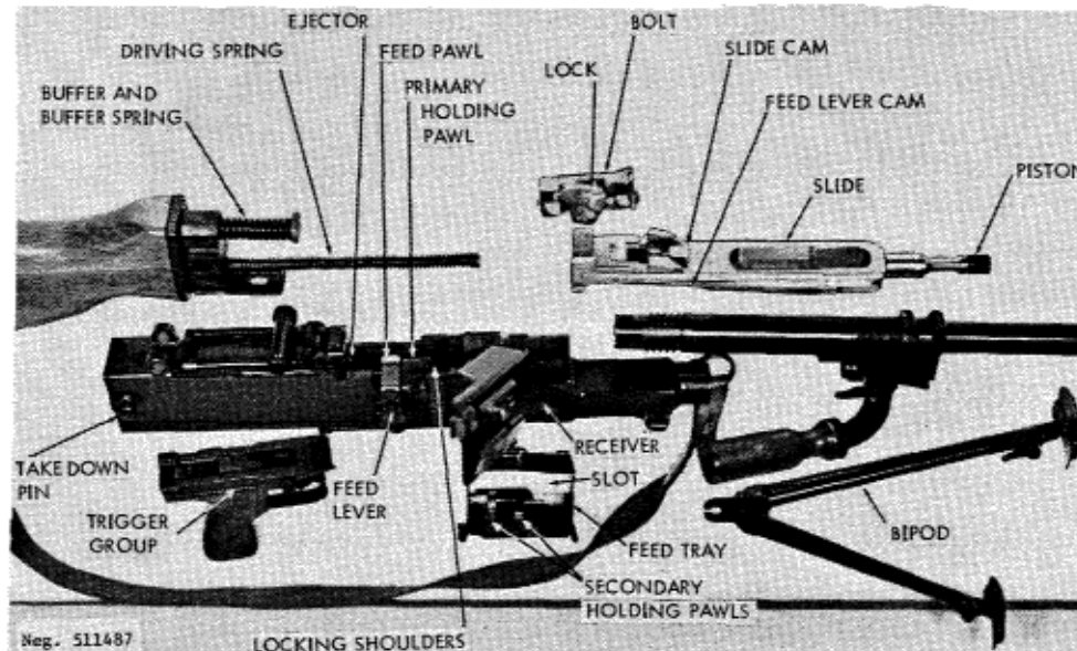
Figure 188. Vz59 full stripped.
