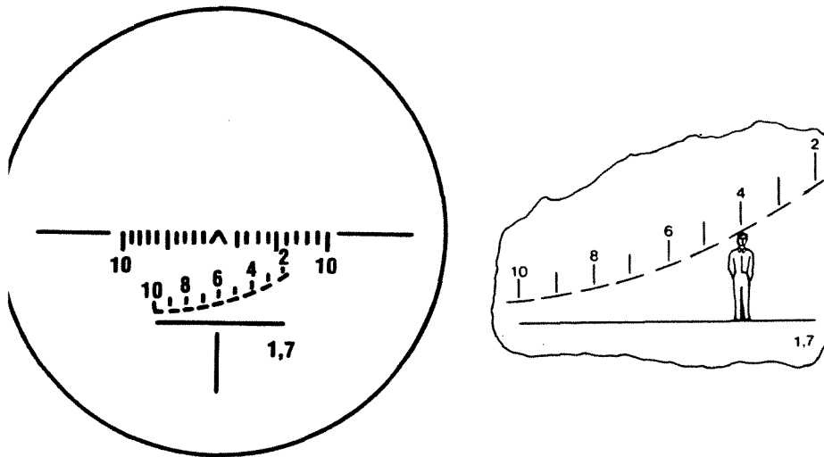
Figure 221.7. Model SPP optical sight reticle.
