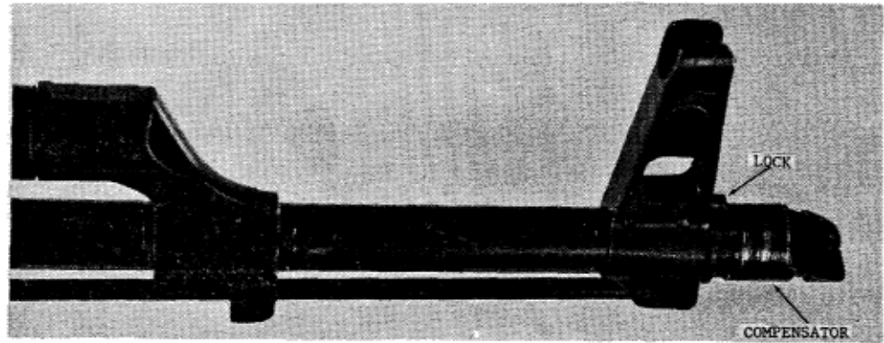
Figure 90. AKM compensator.
