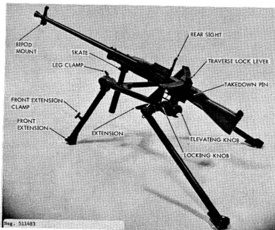
Figure 184. Vz59 general purpose machinegun on tripod.
