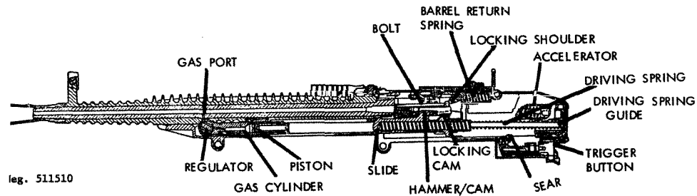
Figure 211. ZB-37 section.
