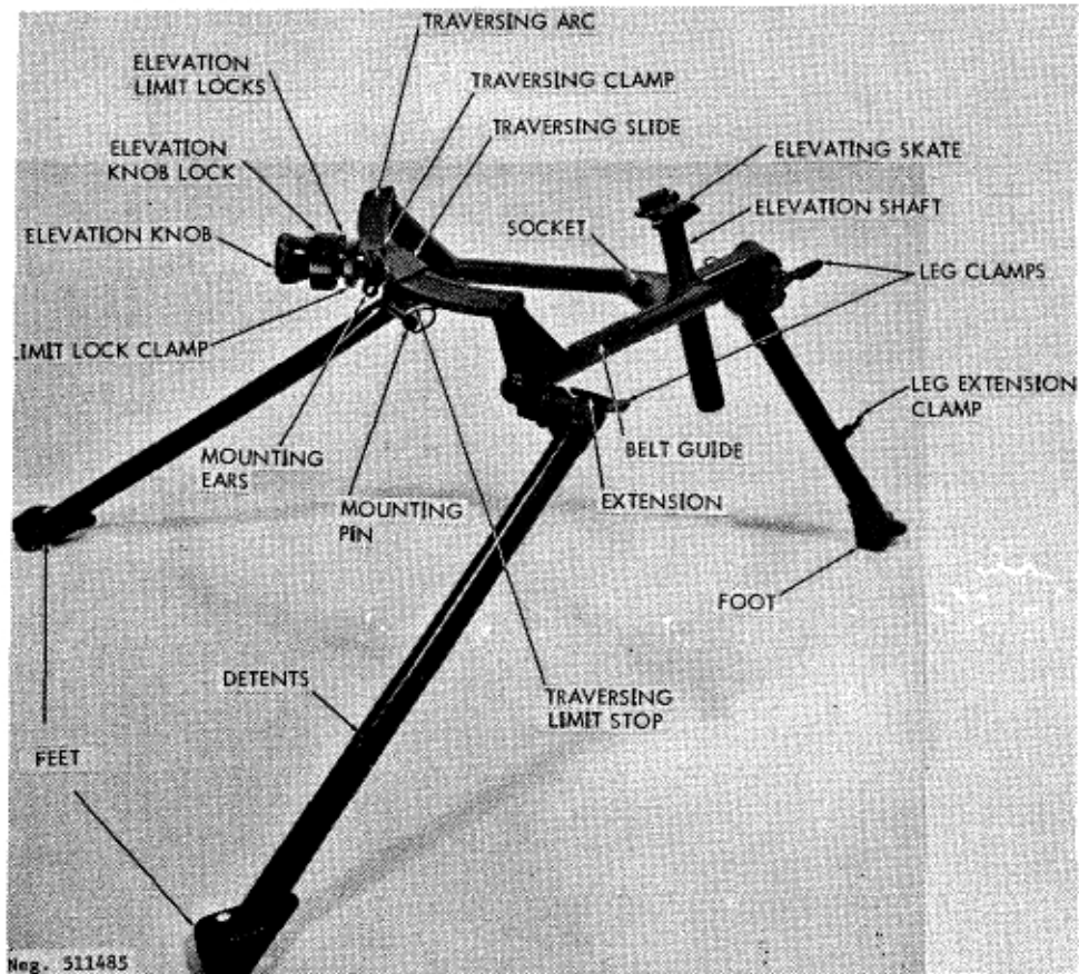
Figure 186. Vz59 tripod.
