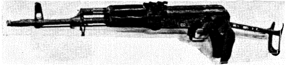
Figure 87.1. North Korean Type 68 assault rifle with compensator.
