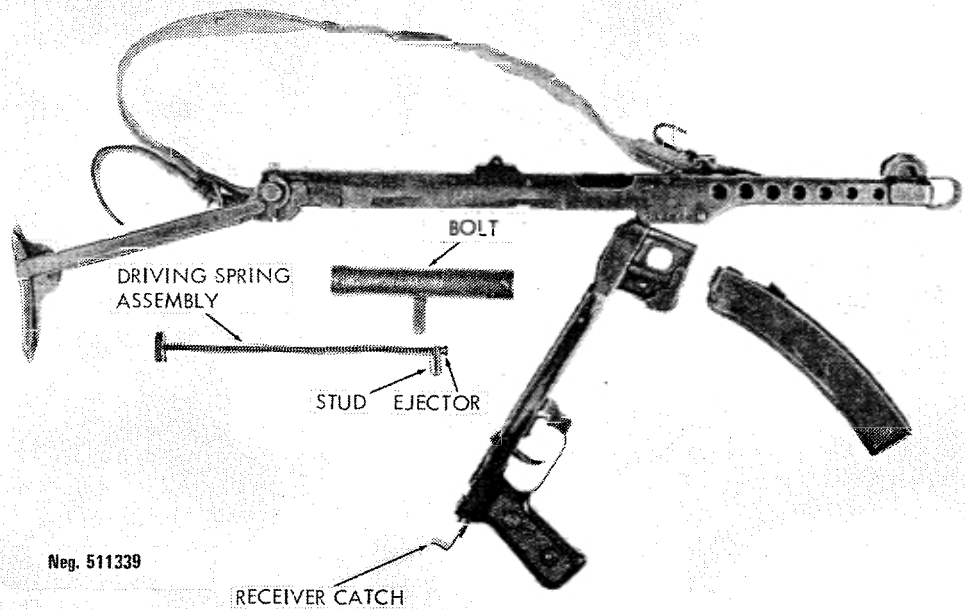
Figure 40. PPS-43 field stripped.
