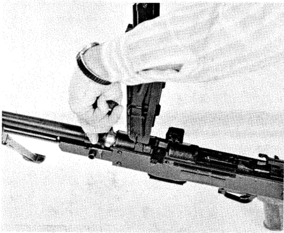
Figure 177. PK barrel change.
