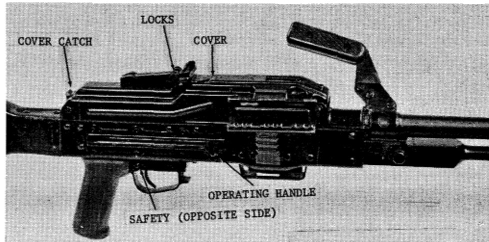
Figure 175. Soviet PKM receiver detail.
