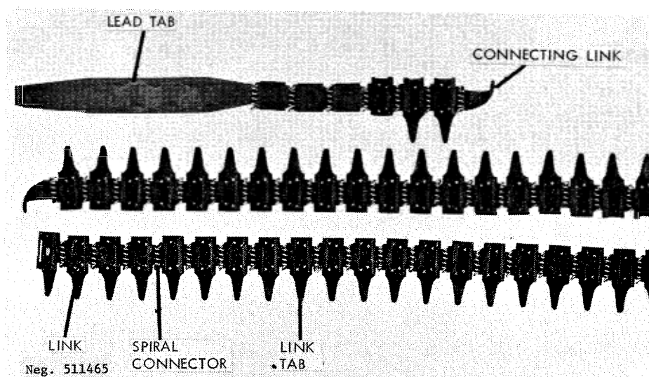
Figure 166. MG34 feed belt.
