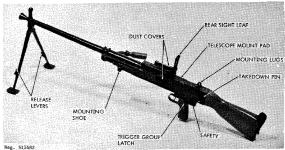
Figure 183. Vz59 light machinegun.
