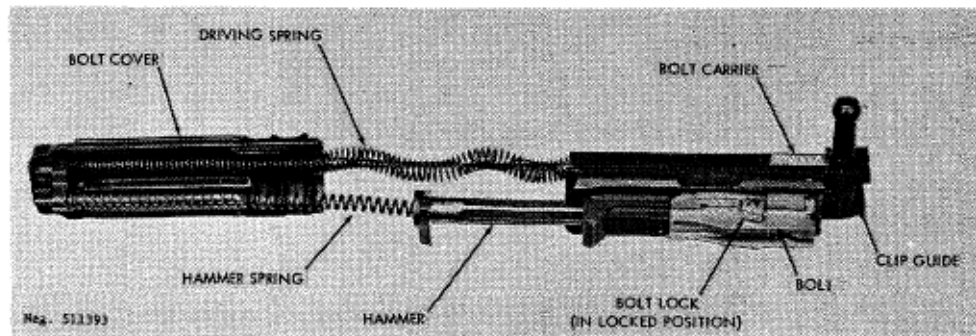
Figure 94. M58 bolt and firing mechanism.
