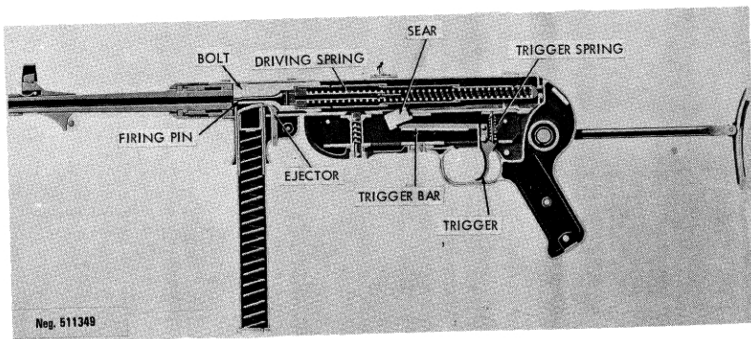
Figure 50. MP40 section.
