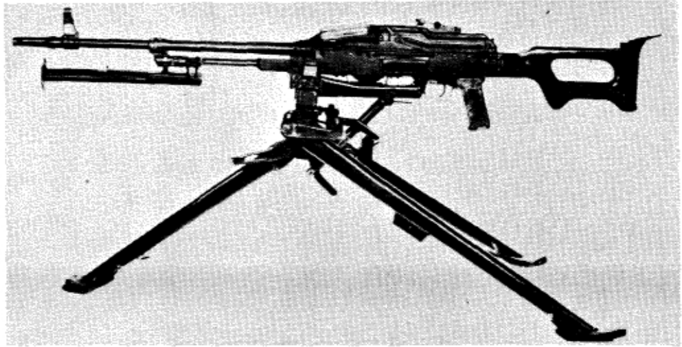
Figure 173.1. The PKMS machinegun.
