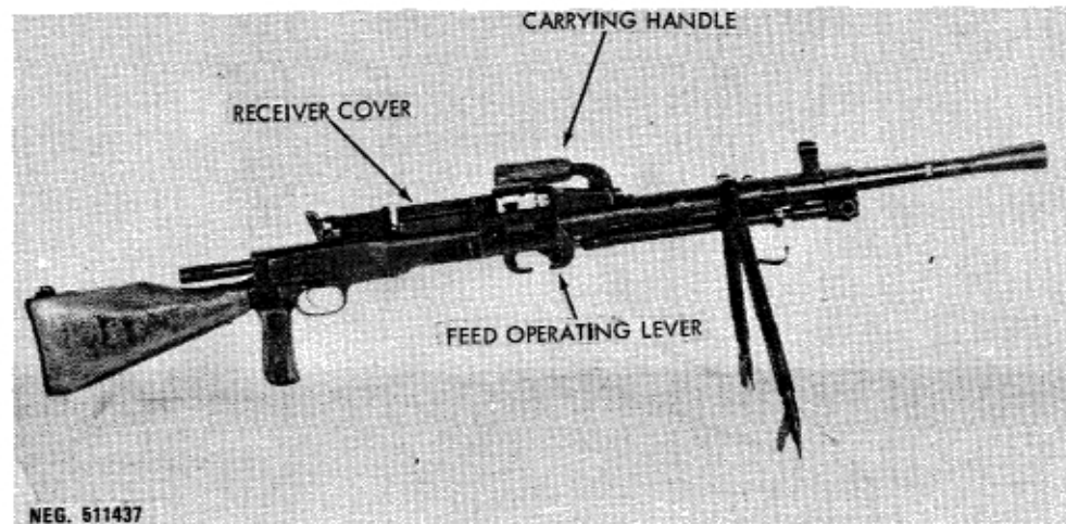
Figure 138. RP-46 company machinegun.
