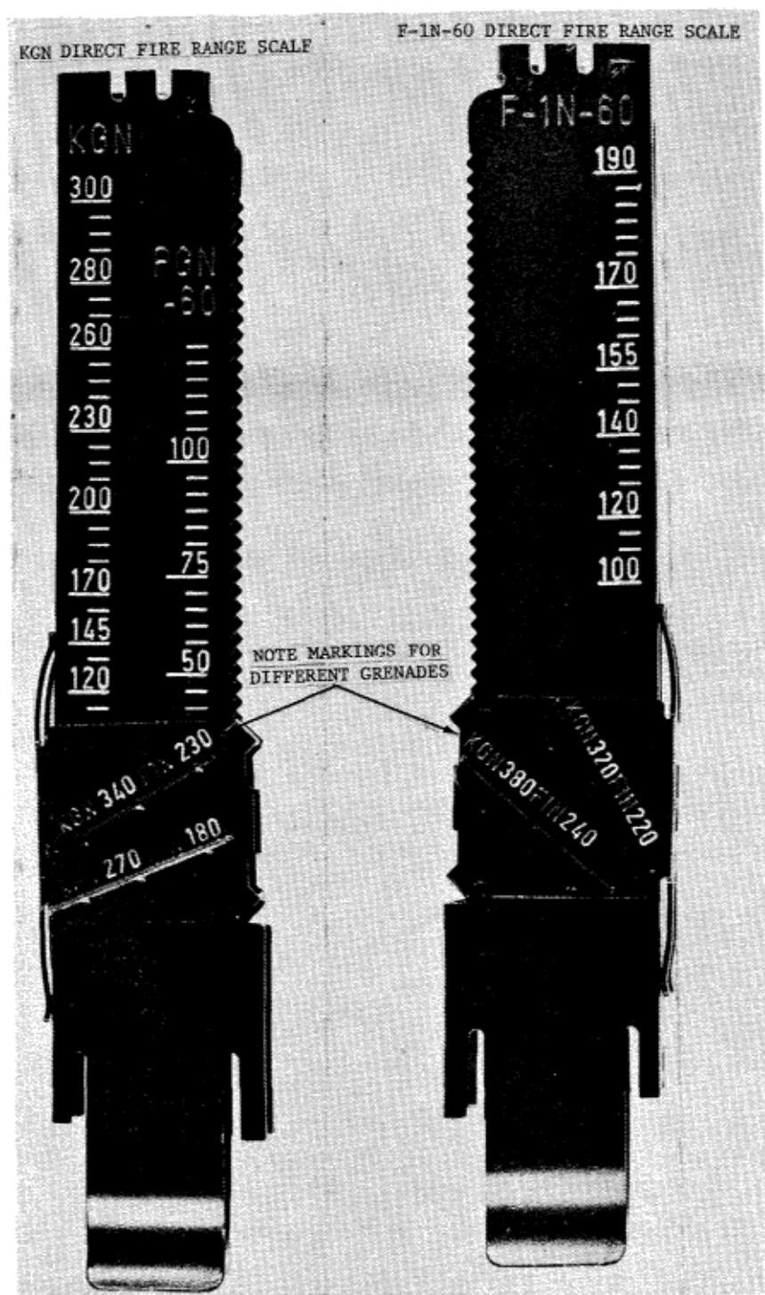
Figure 78.1. Late model grenade sight range scales.
