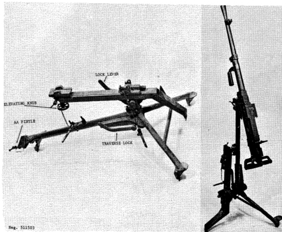
Figure 204. PRC Type 70 tripod.
