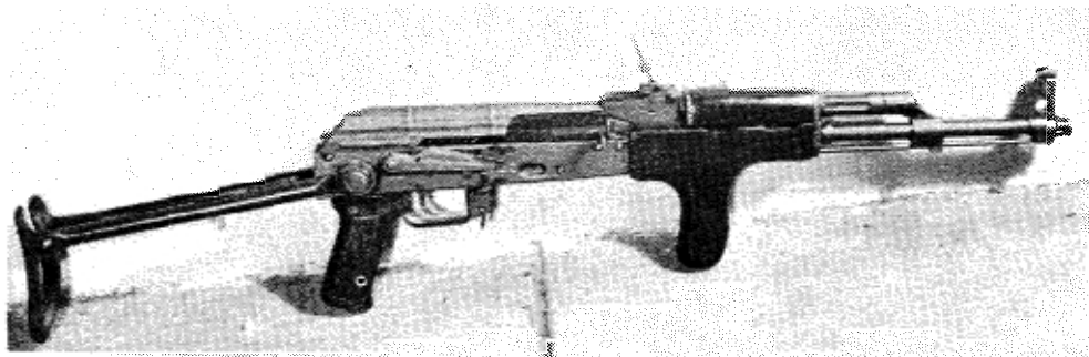
Figure 84.1. Romanian folding-stock AKM.
