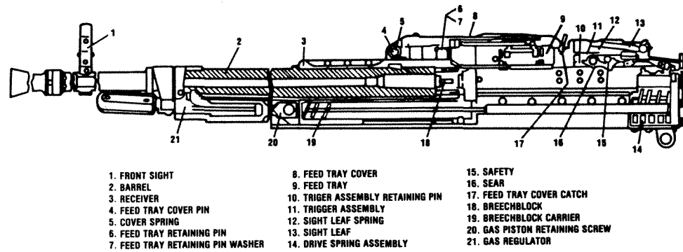
Figure 221.3. NSV 12.7-mm machinegun cross-section.
