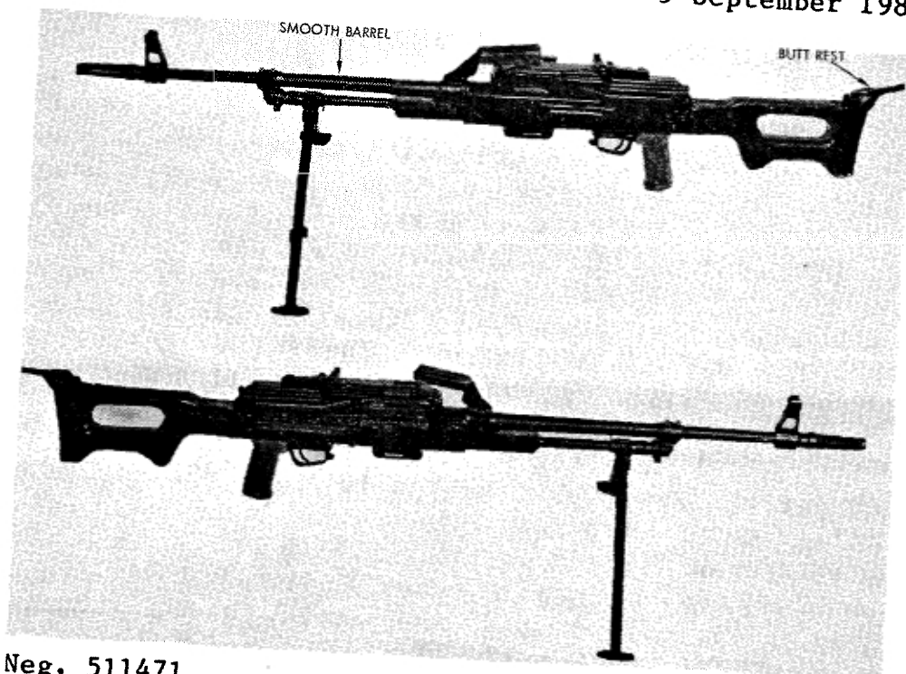
Figure 172. Soviet PKM general purpose machinegun.
