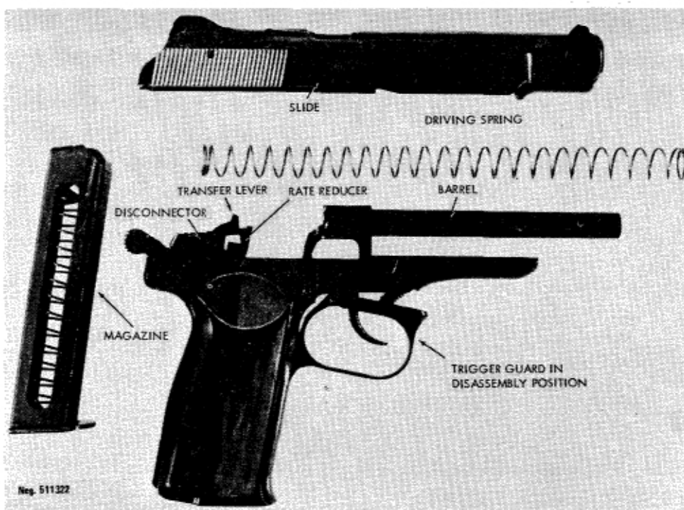
Figure 23. Stechkin, disassembled.
