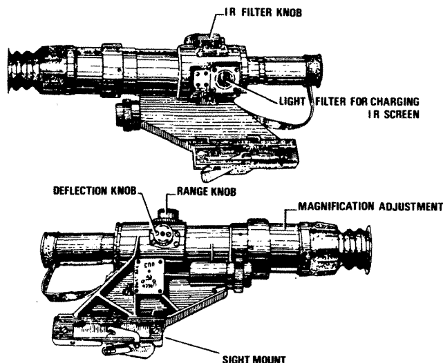
Figure 221.6. Model SPP optical sight
