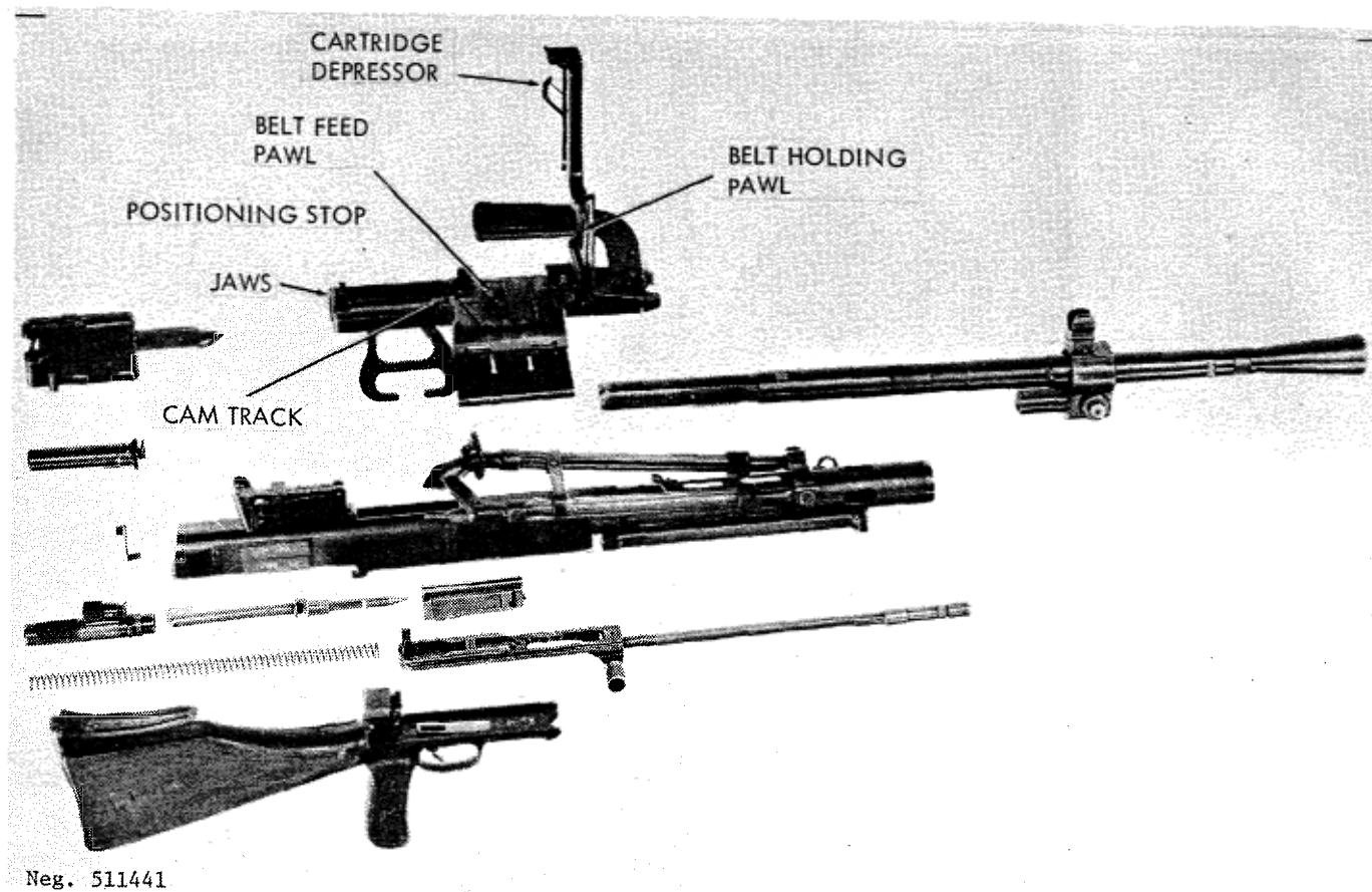
Figure 142. RP-46 field stripped.
