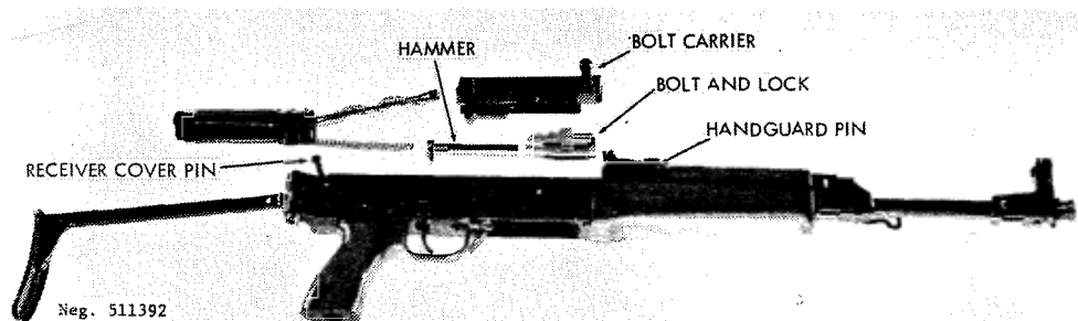
Figure 93. M58V field stripped.
