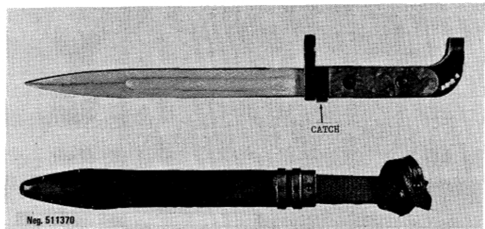
Figure 71. AK-47 bayonet.
