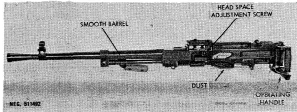
Figure 193. SG-43M heavy machinegun.
