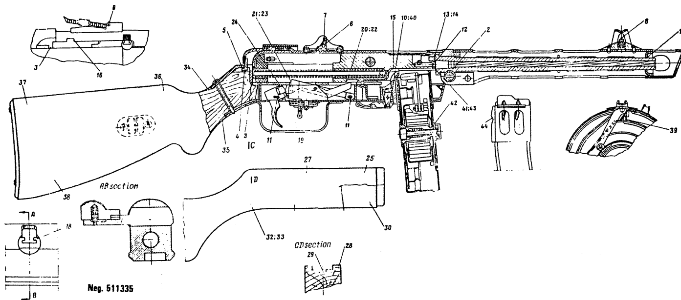
Figure 36. PPSH-41 section.
