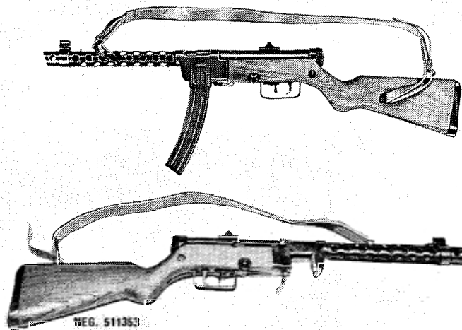
Figure 54. The Yugoslav M49 submachinegun.
