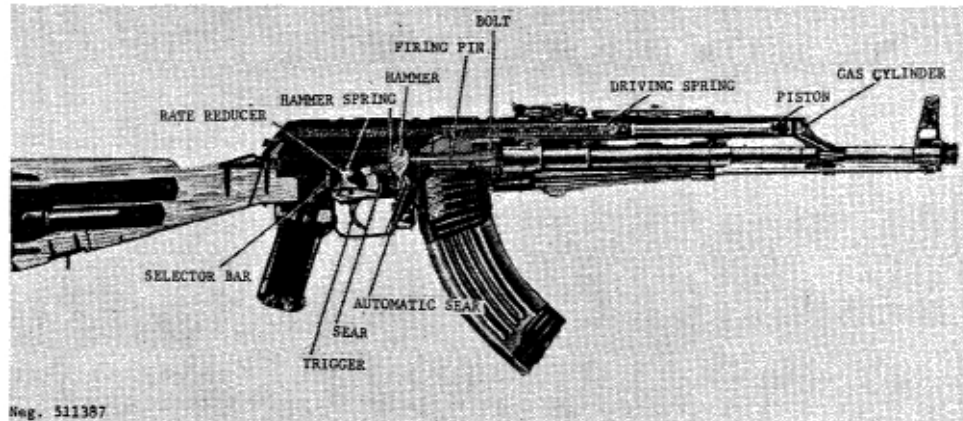
Figure 88. AKM section.
