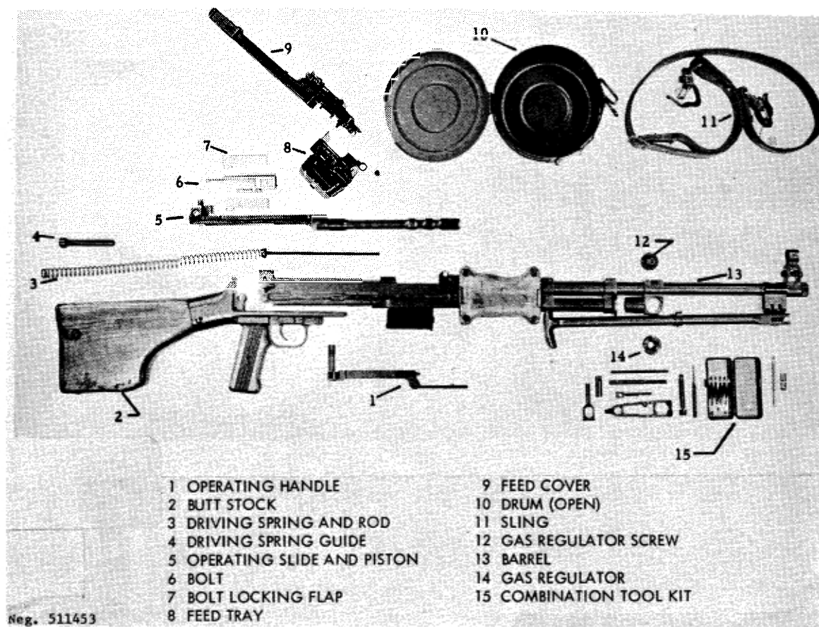
Figure 154. RPD field stripped.
