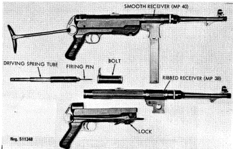
Figure 49. German Model 1938 (bottom) and Model 1940 submachineguns (MP38 and MP40) disassembled.
