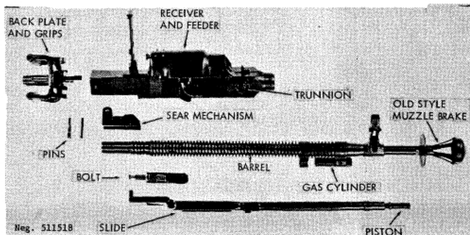
Figure 219. DShK-38 field stripped.
