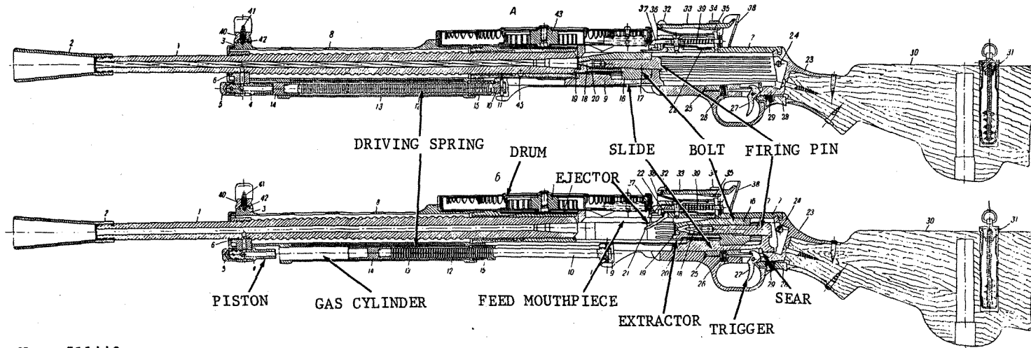
Figure 143. DP section.
