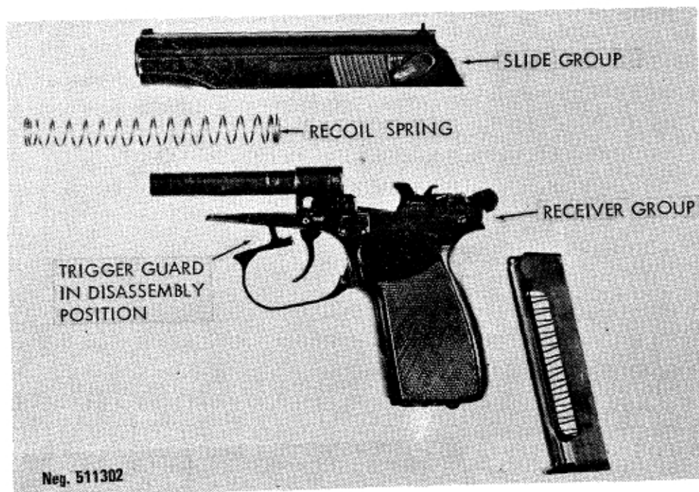
Figure 3. Makarov pistol, field stripped.
