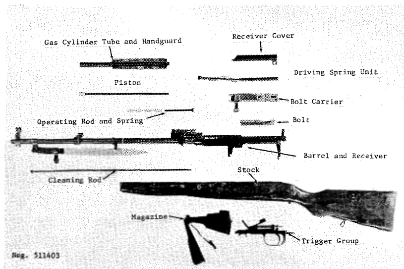
Figure 103. SKS field stripped.
