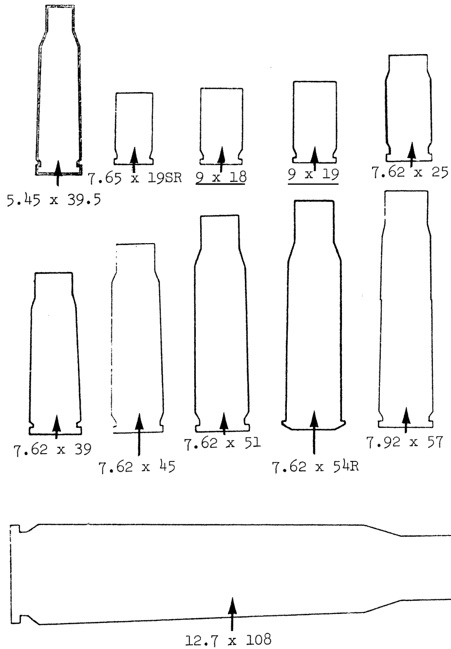
Figure 222. Ammunition identification.
