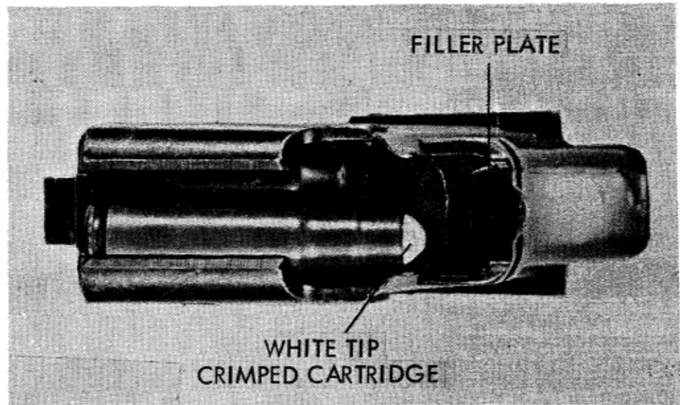
Figure 78. Grenade cartridge and magazine.
