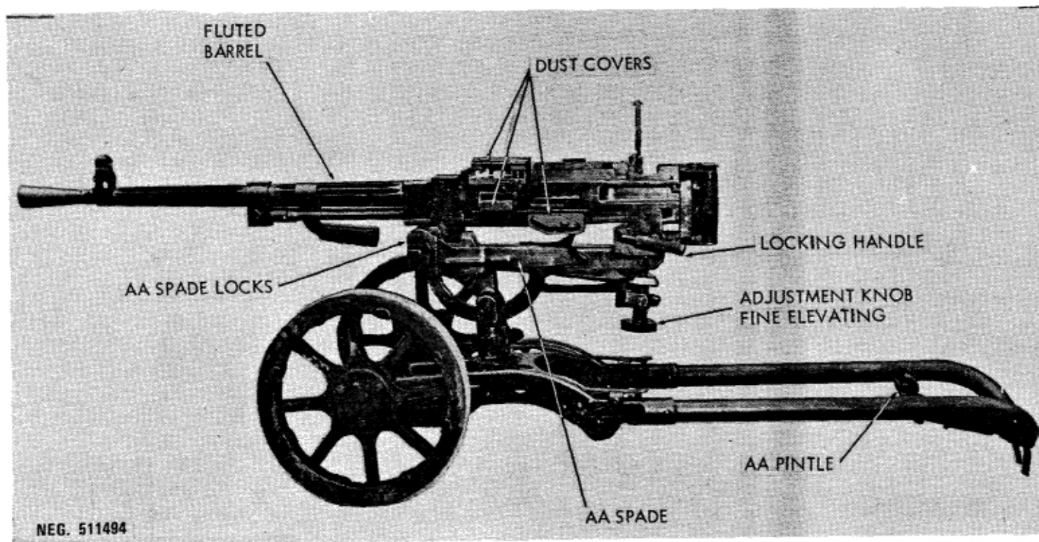
Figure 195. SGMB/PRC Type 57 heavy machinegun.
