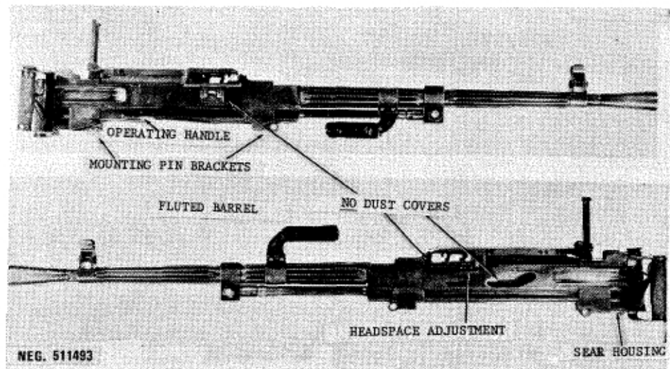
Figure 194. SGM heavy machinegun (early version).
