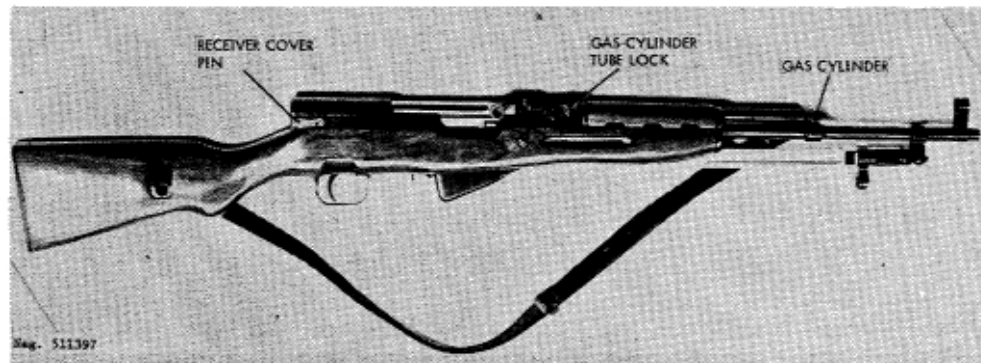
Figure 98. East German Karabiner-S.
