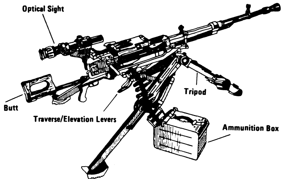
Figure 221.1. Model NSV 12.7-mm machinegun mounted on Model 6T7 tripod.
