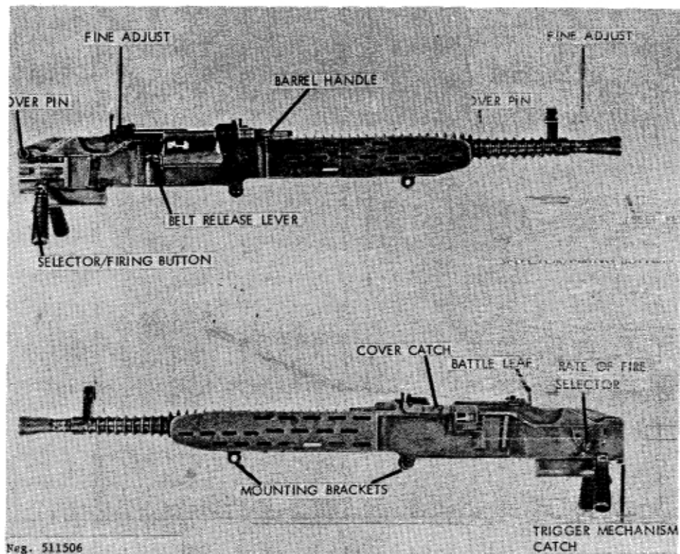
Figure 207. ZB-37 heavy machinegun.
