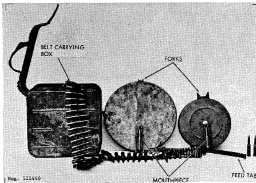
Figure 141. Degtyarev belts and drums.
