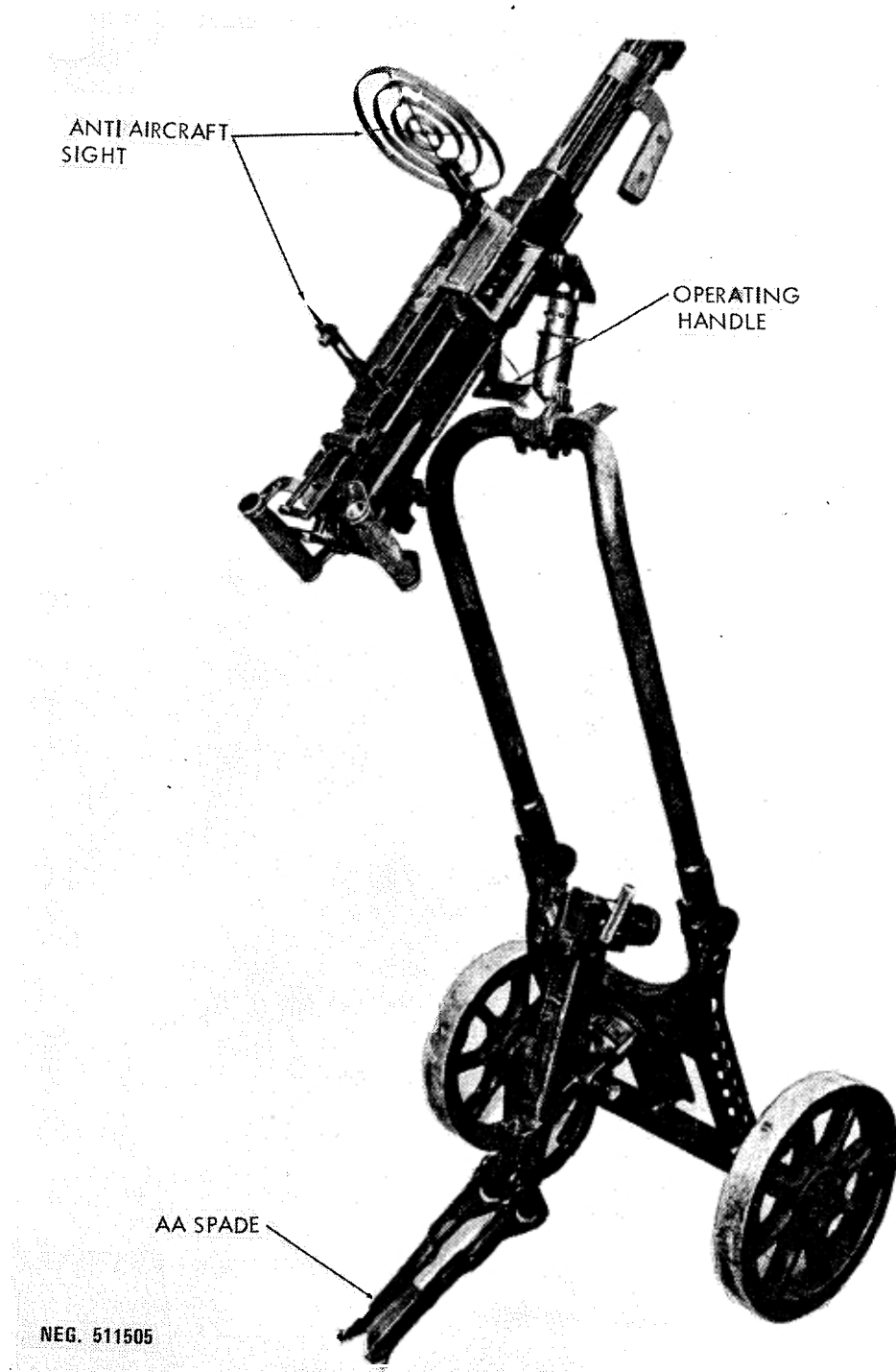
Figure 206. SGMB, antiaircraft position.
