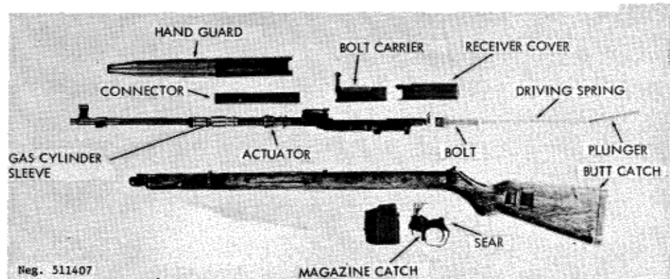
Figure 107. Vz52 field stripped.
