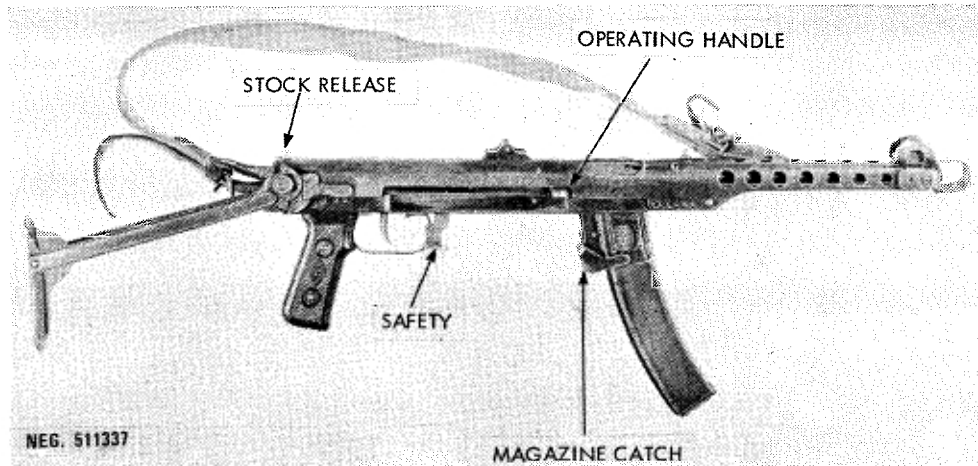
Figure 38. Soviet Model 1943 submachinegun (PPS-43).
