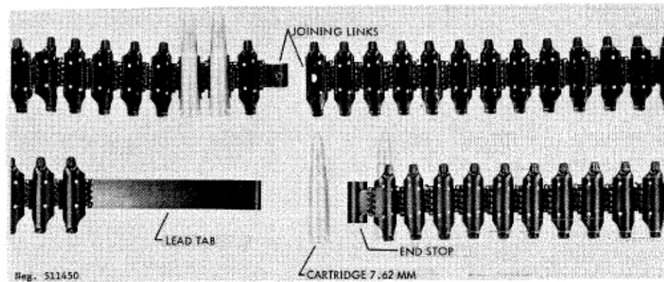
Figure 151. RPD feed belt.
