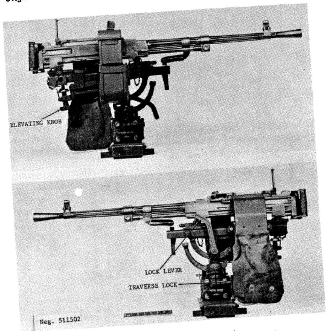
Figure 203. Early SGM on vehicular mount.
