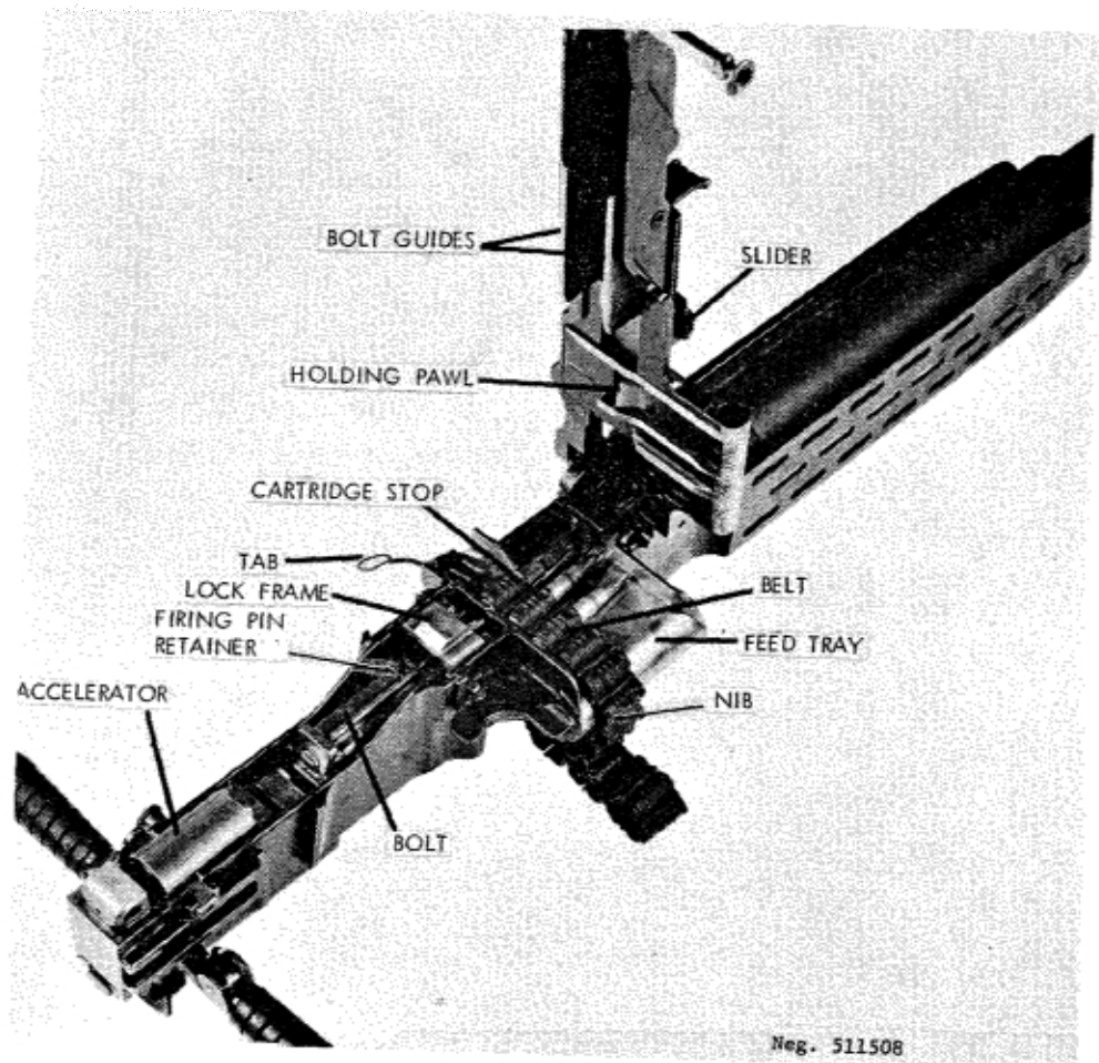
Figure 209. Loading the ZB-37.
