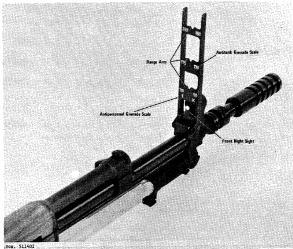
Figure 102. M59/66 grenade sight erected.
