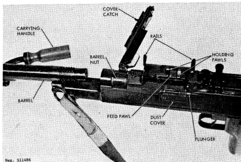
Figure 187. Vz59 barrel change.
