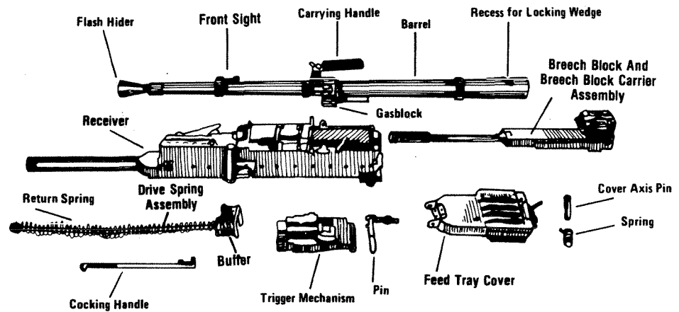
Figure 221.4. NSV 12.7-mm machinegun disassembled.
