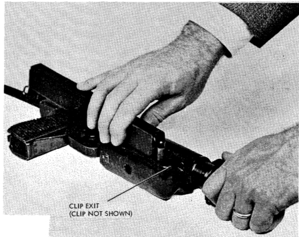
Figure 46. Using magazine filler to load magazine.
