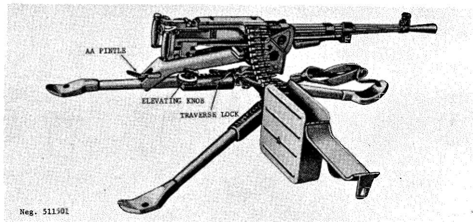
Figure 202. SGM Sidorenko-Malinovski tripod.
