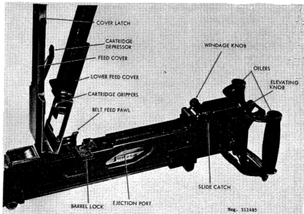
Figure 196. SG-43 receiver detail.
