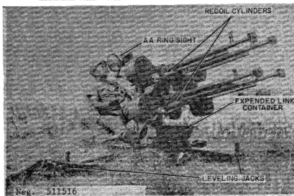
Figure 217. Czechoslovak quad-mounted M54 heavy machinegun.
