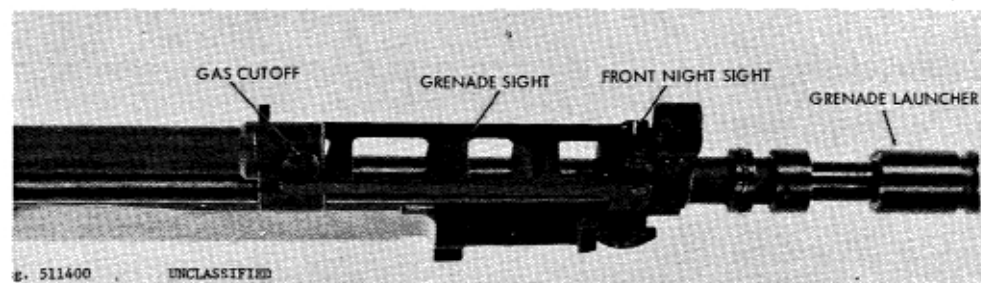
Figure 100. M59/66 gas cutoff.
