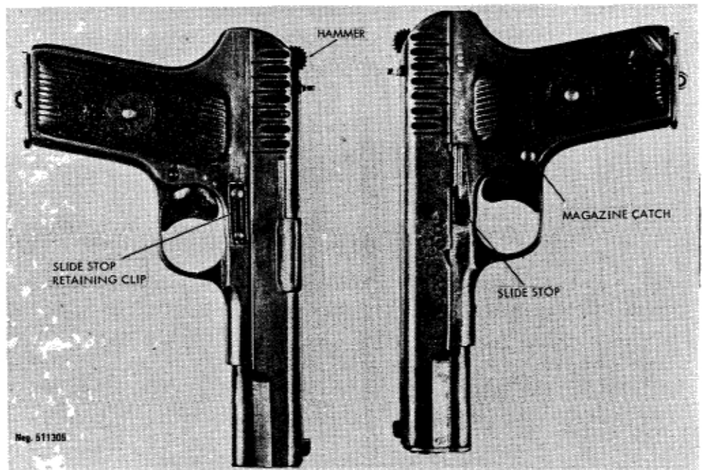
Figure 6. Soviet Tokarev pistol (TT-33).
