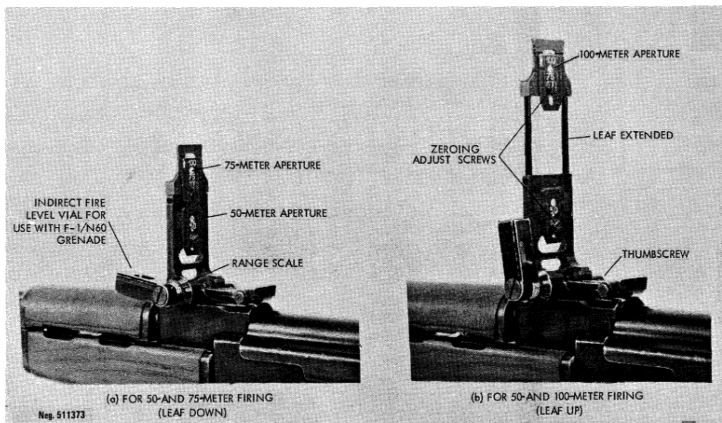
Figure 74. Grenade launching sights.
