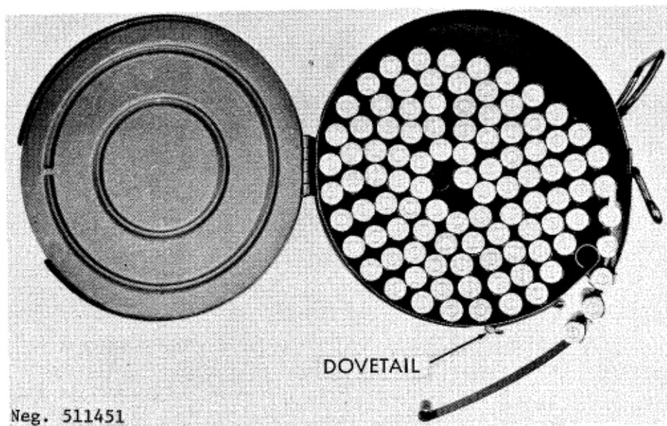
Figure 152. RPD drum.
