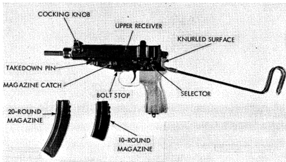
Figure 25. Czechoslovak Vz61 "Skorpion" machine pistol.
