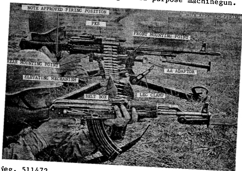
Figure 173. Soviet PKS machinegun.
