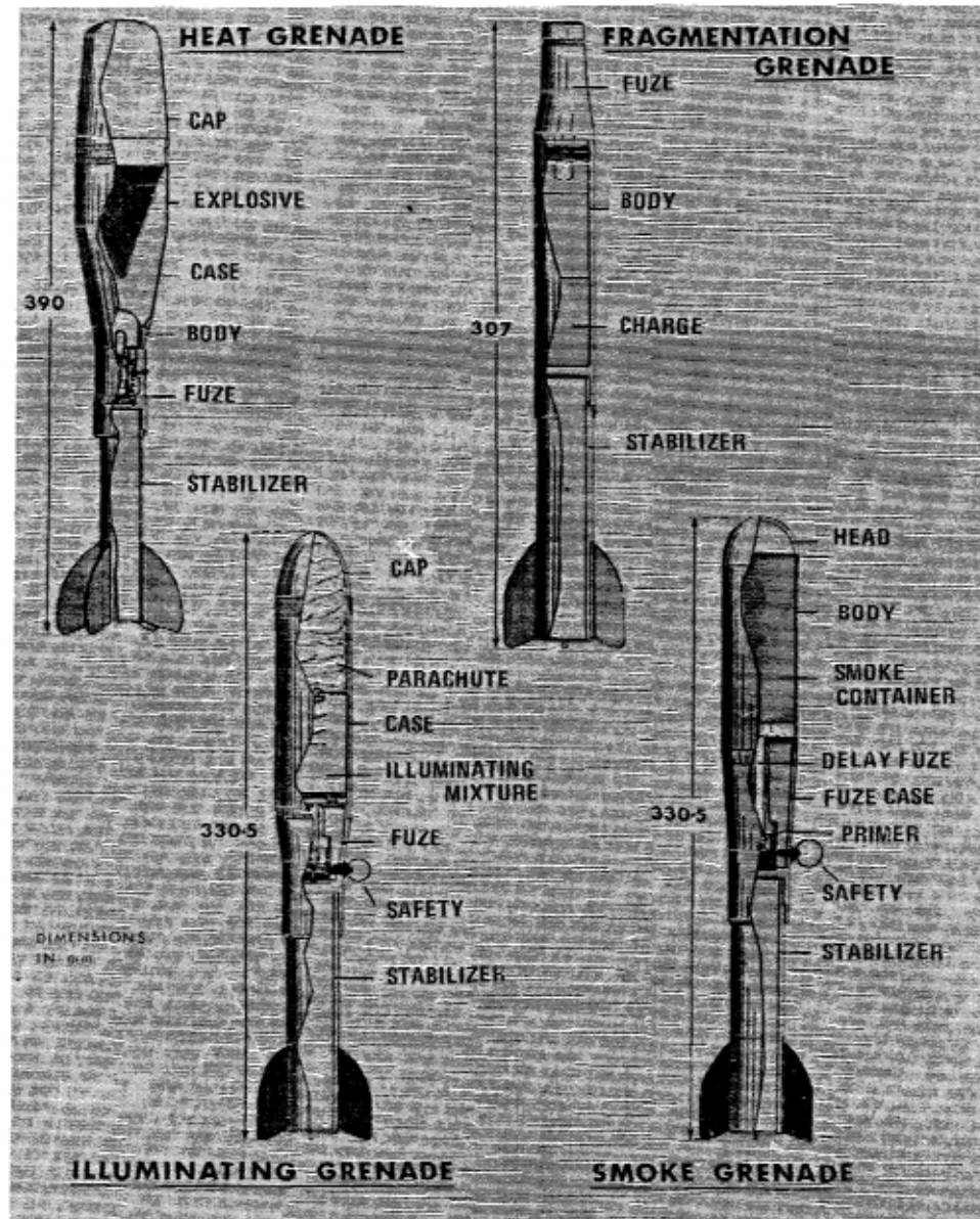
Figure 77. Yugoslav rifle grenades.
