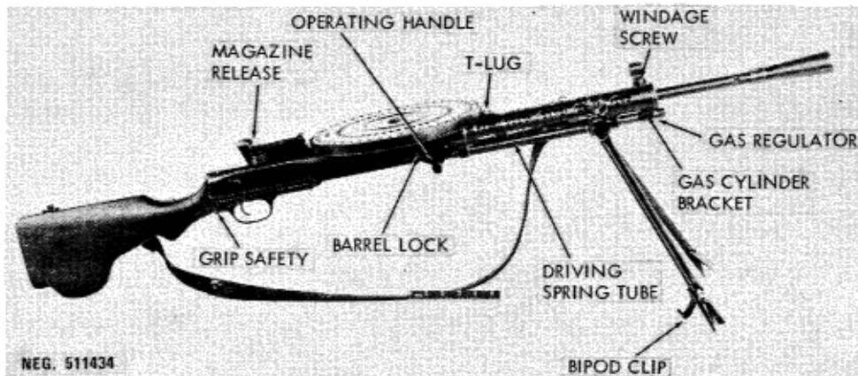
Figure 135. Degtyarev DP light machinegun.
