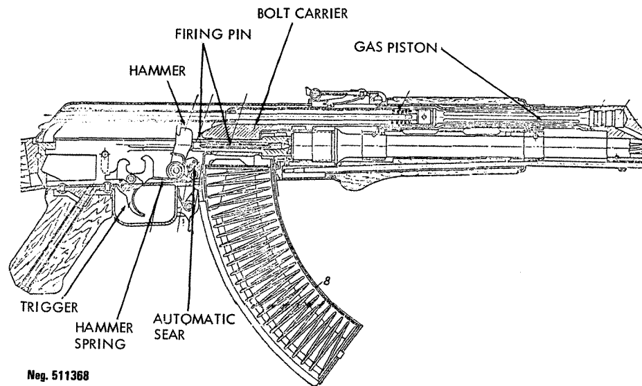
Figure 69. AK-47 section.
