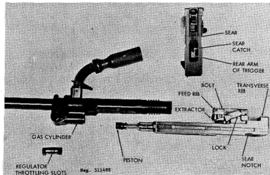
Figure 189. Vz59 mechanism.
