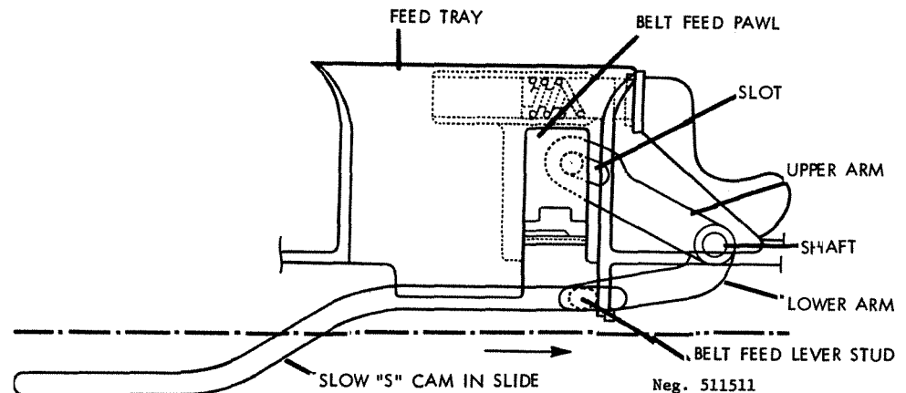
Figure 212. ZB-37 feed mechanism.
