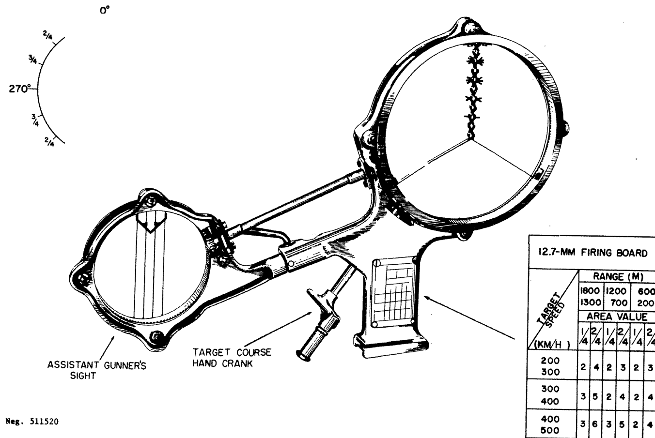
Figure 221. M1943 antiaircraft sight.
