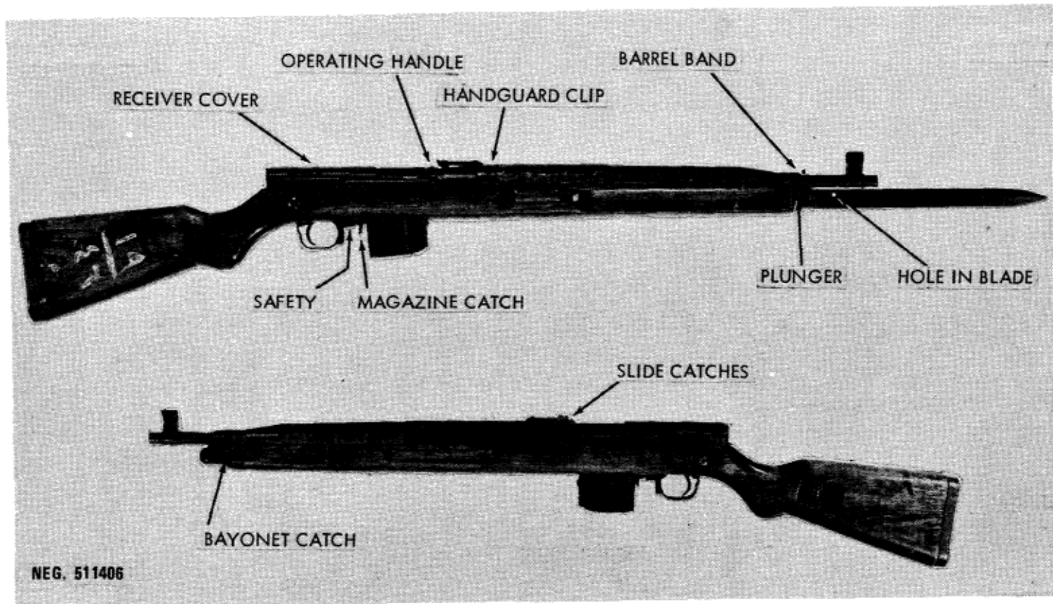
Figure 106. Czechoslovak M52 or M52/57 rifle.
