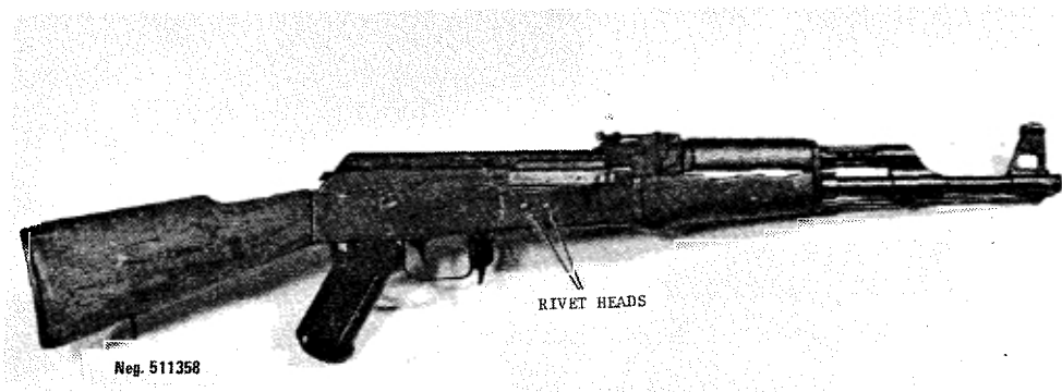
Figure 59. Stamped receiver AK-47.
