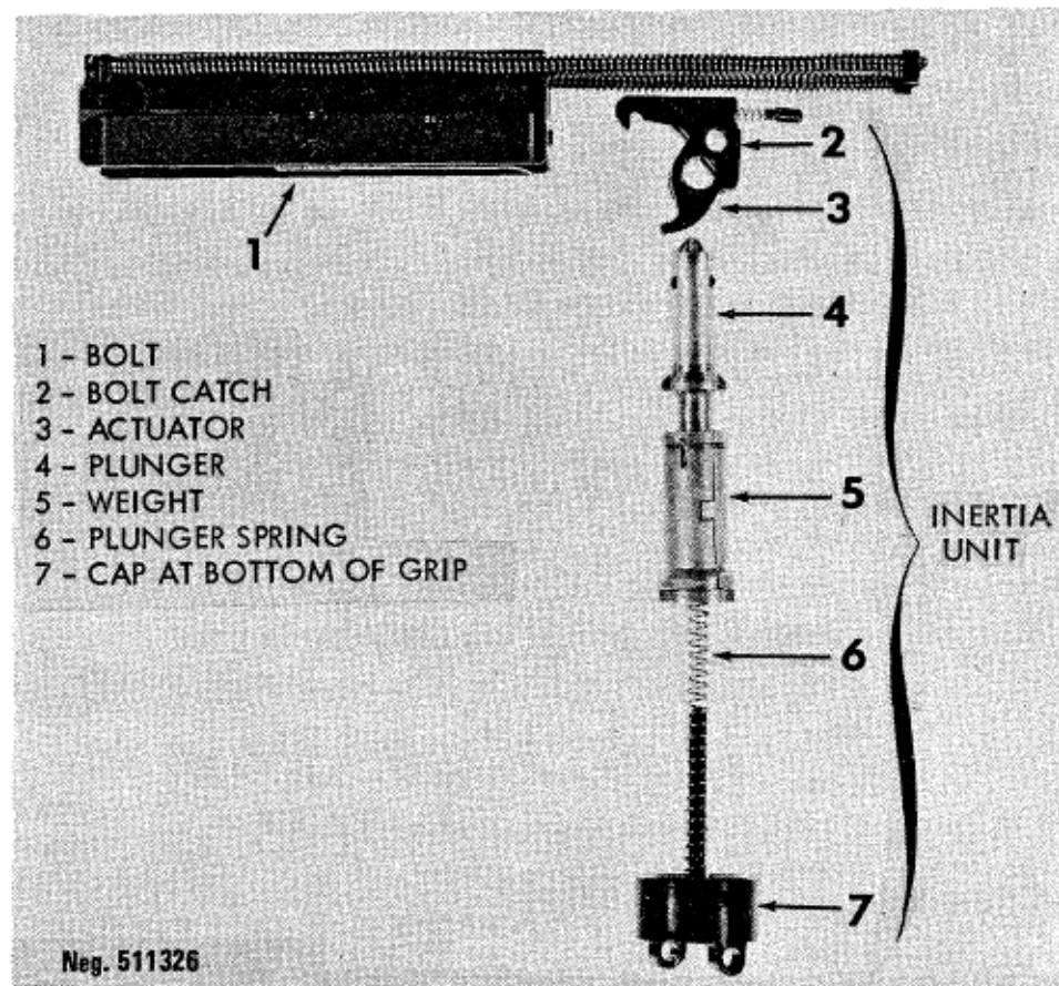
Figure 27. Vz61 rate reducer.
