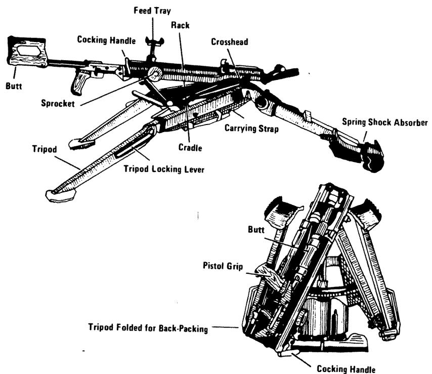
Figure 221.5. Model 6T7 tripod in firing and travel positions.
