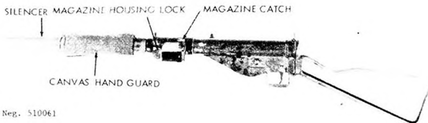
Figure 62. Sten Mark 2S silenced submachinegun.
