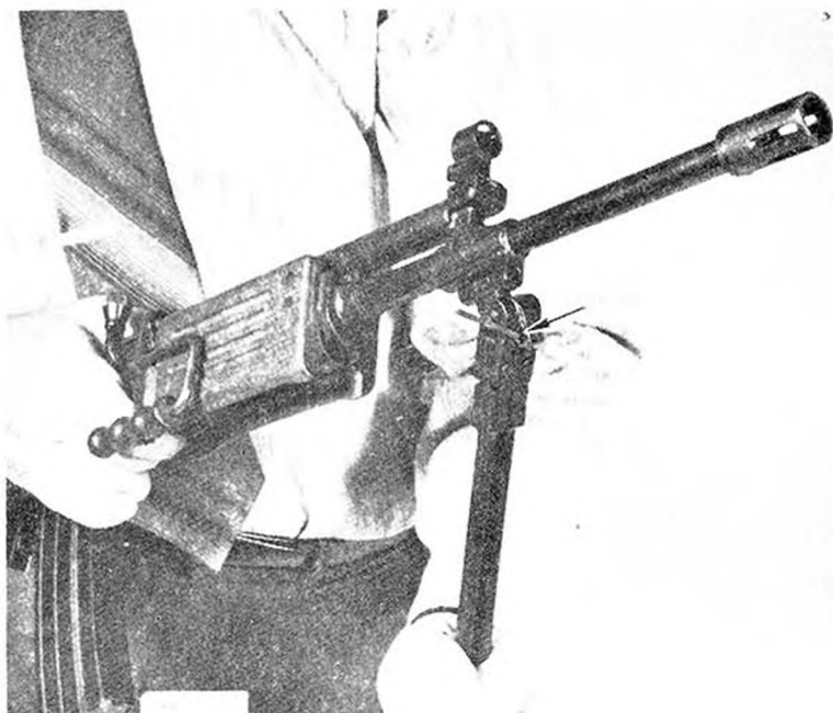
Figure 93. Using the Galil to cut wire.
