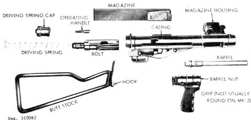
Figure 63. Sten Mark 2 submachinegun, disassembled.
