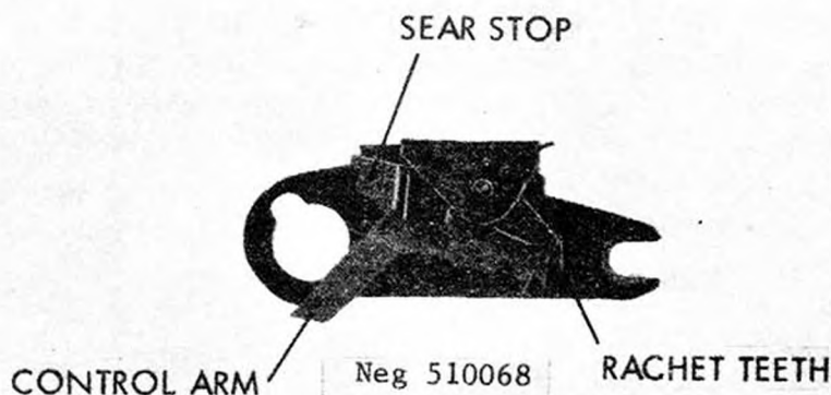
Figure 69. C.A.L. burst limiter.
