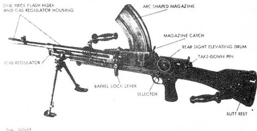
Figure 150. Mark 1 Bren.
