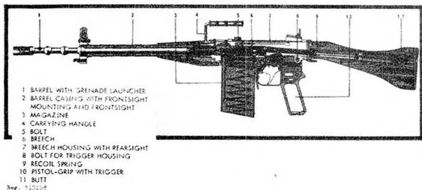
Figure 129. SIG 510-4 section.
