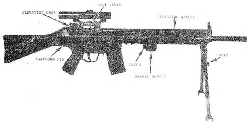
Figure 169. West German HK 13 light machinegun.
