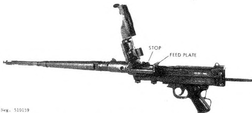
Figure 160. AAT-52 tank machinegun.
