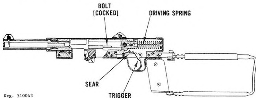
Figure 44. M45b section.
