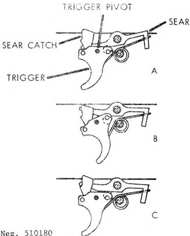
Figure 181. MG-1 trigger functioning.
