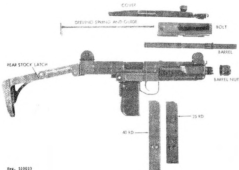
Figure 34. UZI submachinegun, field stripped.
