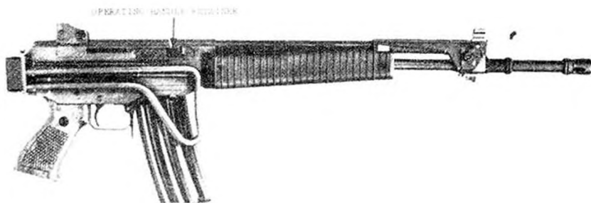
Figure 98. Beretta M70/.223 rifle with folding stock (early model).
