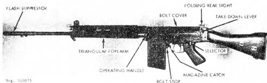
Figure 76. British L1A1 rifle.
