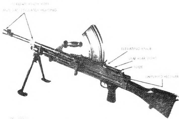
Figure 151. Mark 2 Bren.
