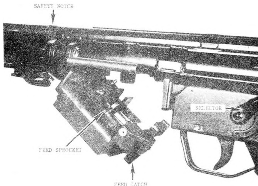
Figure 171. West German HK 21A1 feeder.
