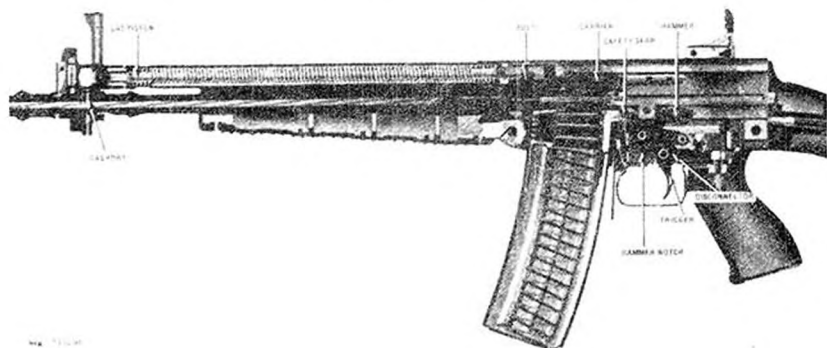
Figure 101. Beretta M70/.223 section.
