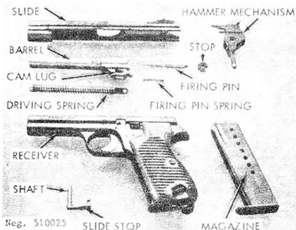
Figure 26. M49 pistol, disassembled.
