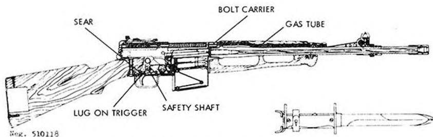
Figure 119. M.A.S. 49/56 section.
