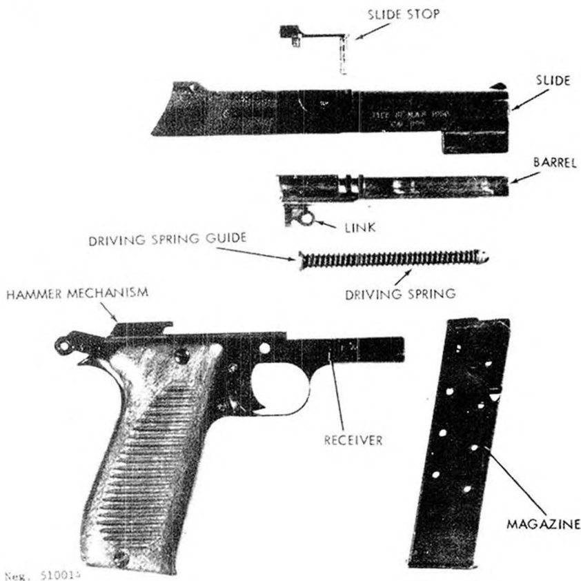
Figure 15. Model 1950 pistol, disassembled.
