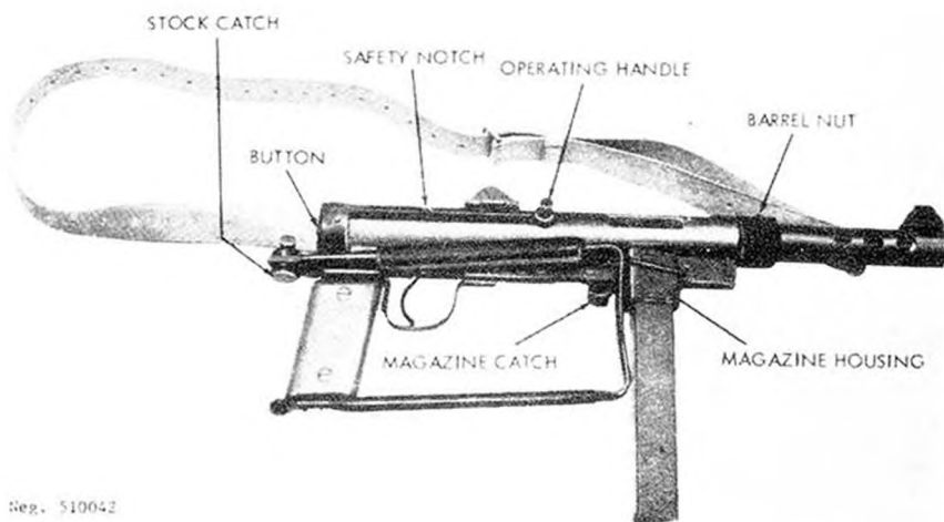
Figure 43. Egyptian Port Said submachinegun.
