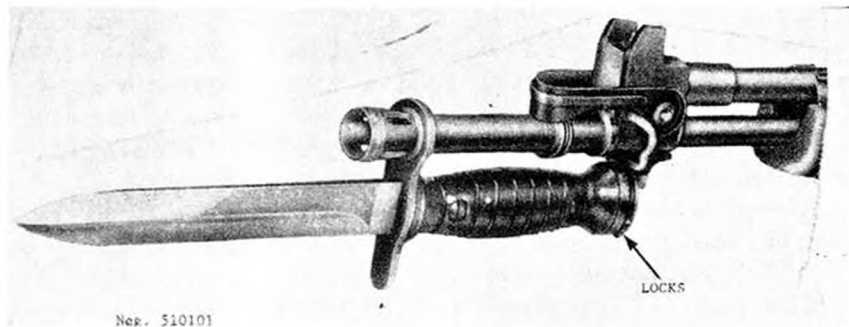
Figure 102. Beretta M70/.223 bayonet.
