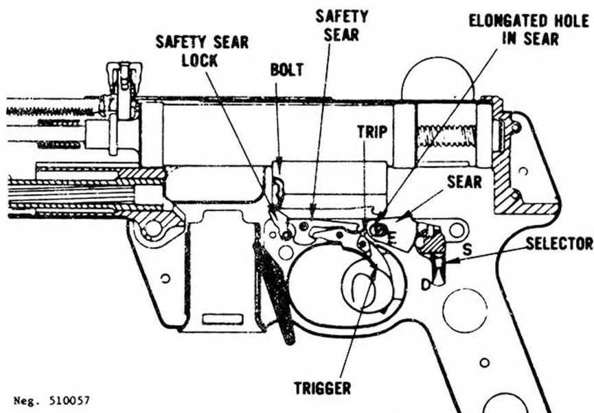
Figure 58. Walther MP-K or MP-L section.
