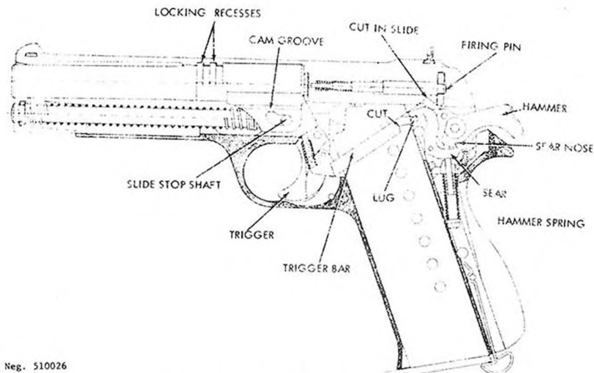
Figure 27. M49 pistol, section.
