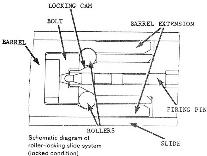
Figure 23. P9 bolt functioning.
