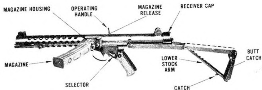
Figure 29. British L2A3 submachinegun.
