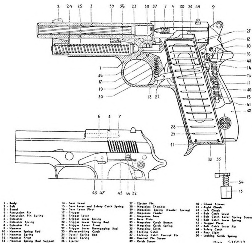
Figure 13. Beretta Model 1951 section.
