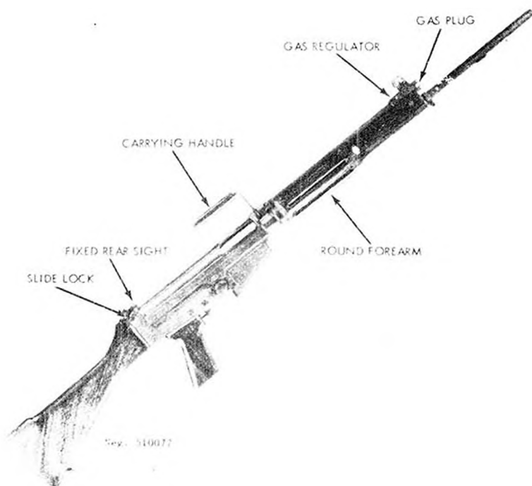
Figure 78. FN/FAL rifle, early version.
