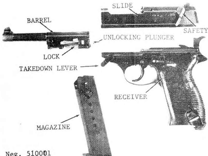
Figure 2. P1 pistol, disassembled.
