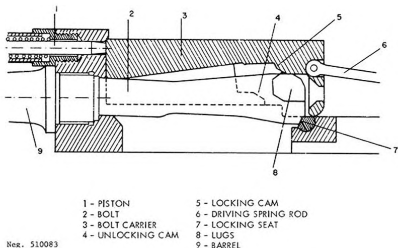
Figure 84. FN/FAL bolt mechanism.
