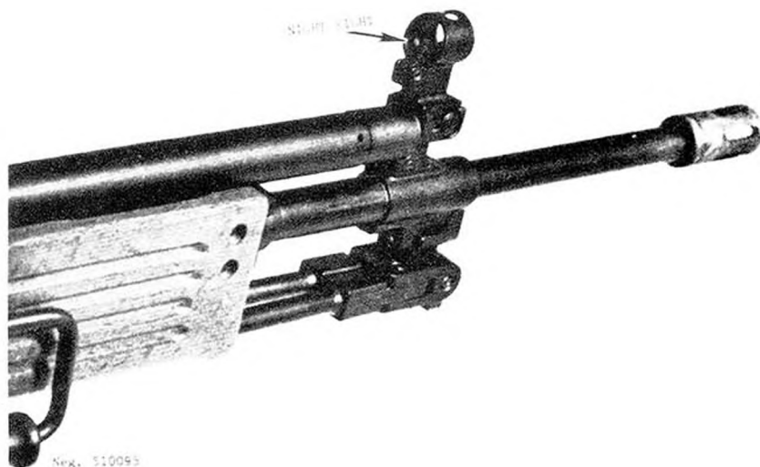
Figure 96. Galil front night sight.
