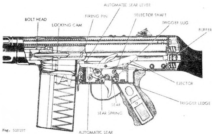
Figure 108. G3 rifle section.
