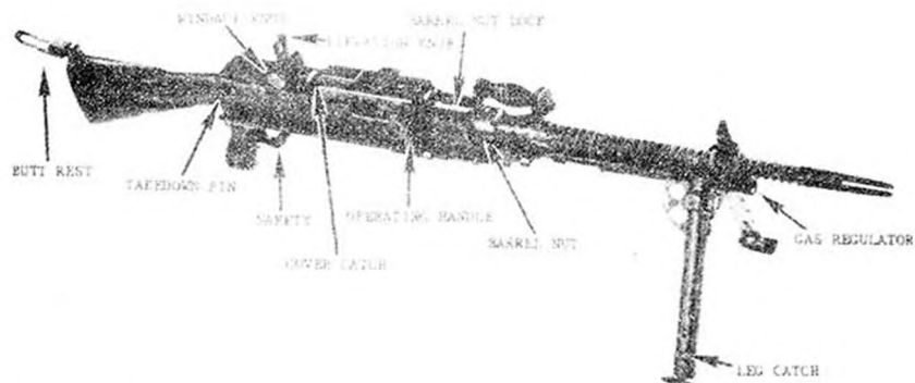
Figure 182. Japanese Type 62 machinegun.
