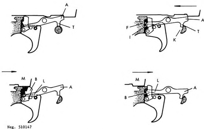
Figure 148. M.A.G. trigger functioning.
