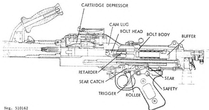
Figure 163. AA-52 section.
