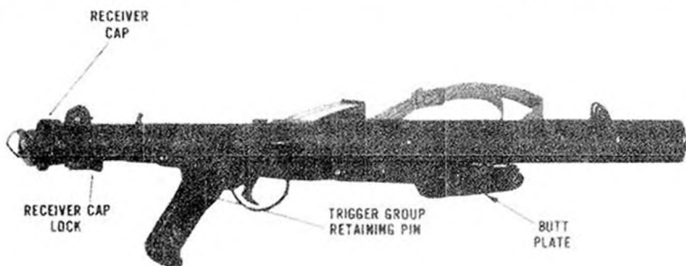
Figure 30. British L34A1 silenced submachinegun.
