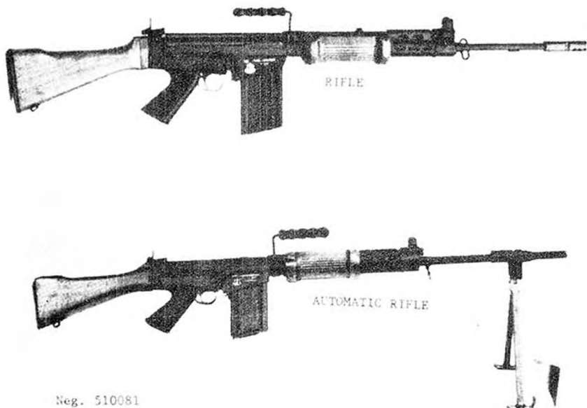
Figure 82. Israeli FN/FAL rifle and automatic rifle.
