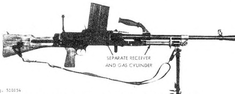
Figure 155. Nationalist Chinese Type 41 Bren.
