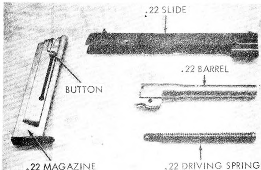
Figure 28. M49 pistol .22 caliber conversion unit.
