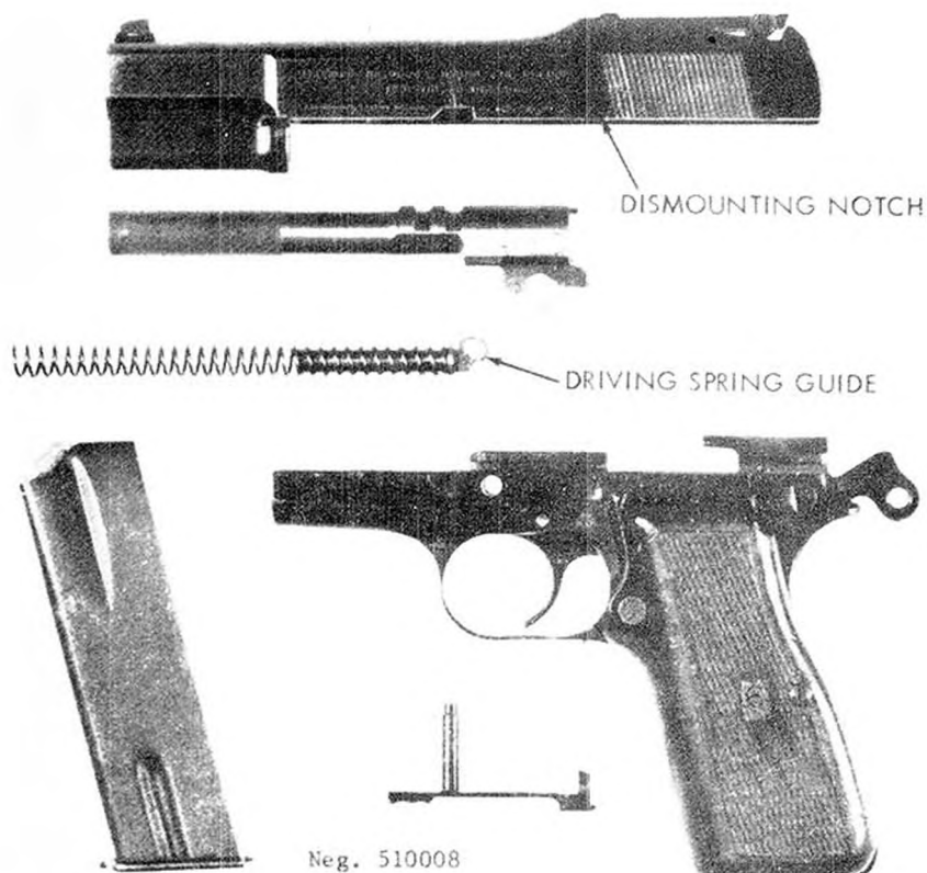
Figure 9. High Power pistol, disassembled.
