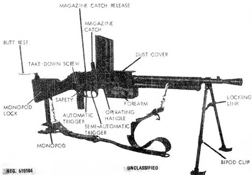
Figure 165. French Model 24/29 light machinegun.
