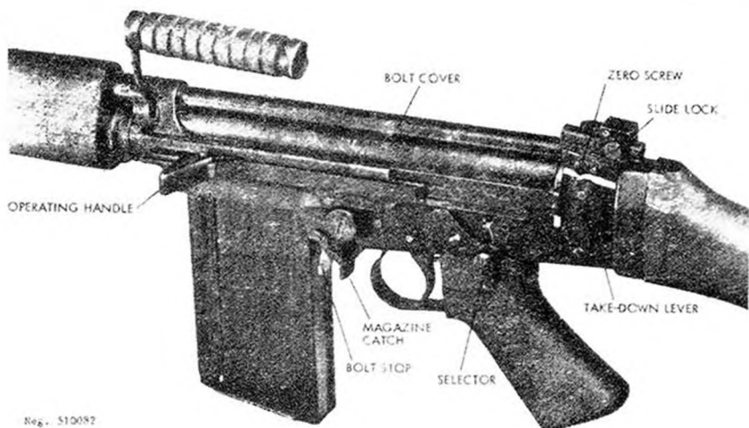
Figure 83. L1A1 receiver details.
