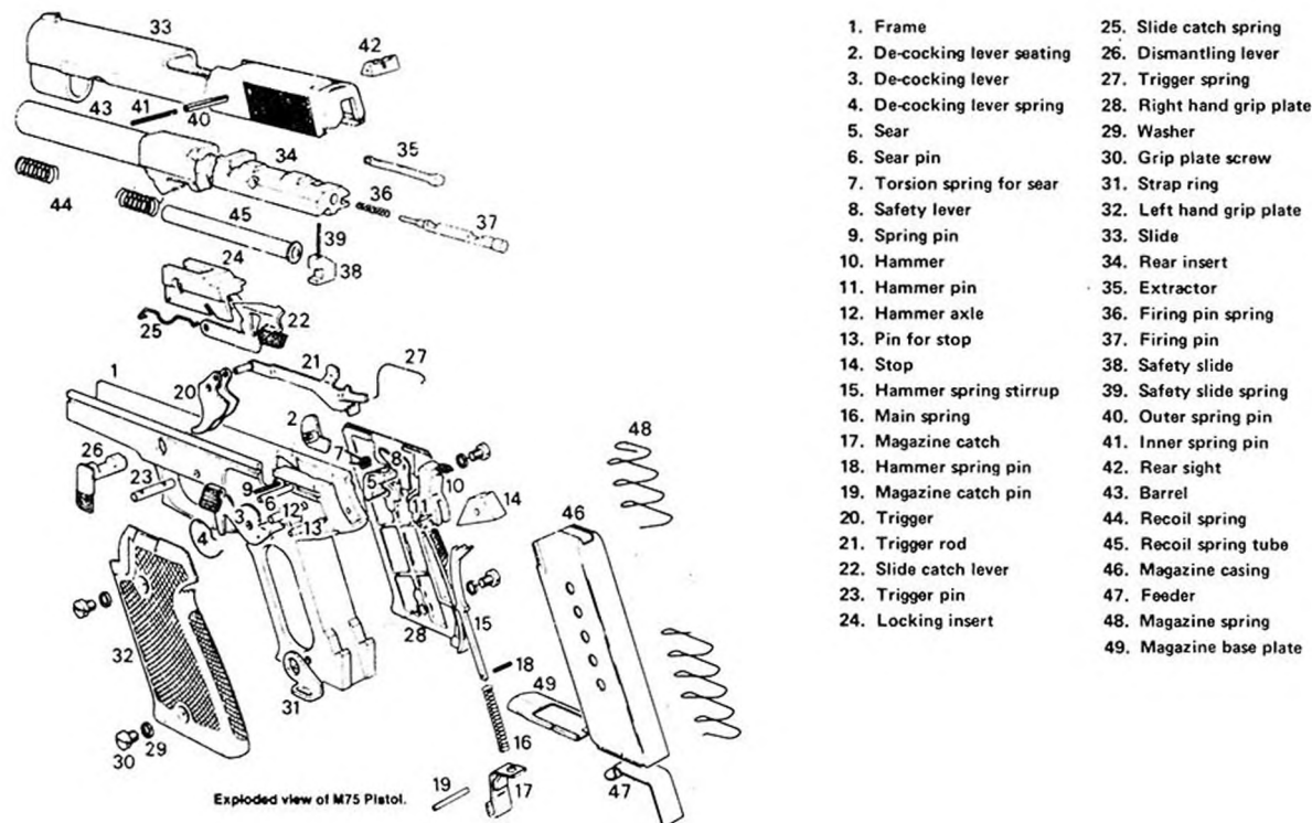
Figure 28.1.1. Swiss 9-mm Model 75 pistol, exploded view.
