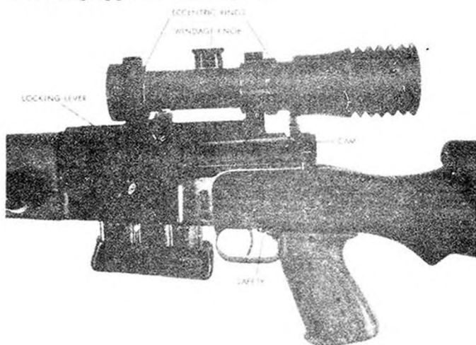
Figure 135. APX 804 telescopic sight.
