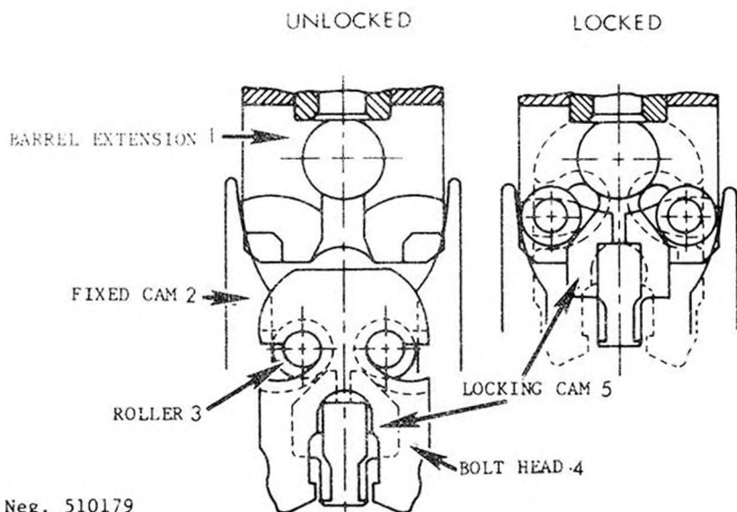
Figure 180. MG-1 bolt functioning.
