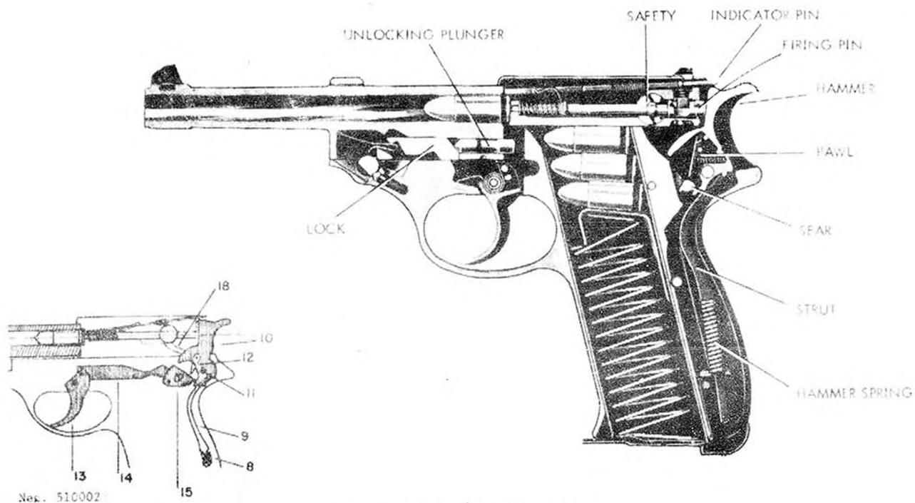
Figure 3. P1 pistol, section.
