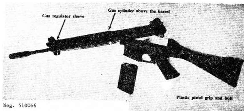
Figure 67. C.A.L. open for disassembly.
