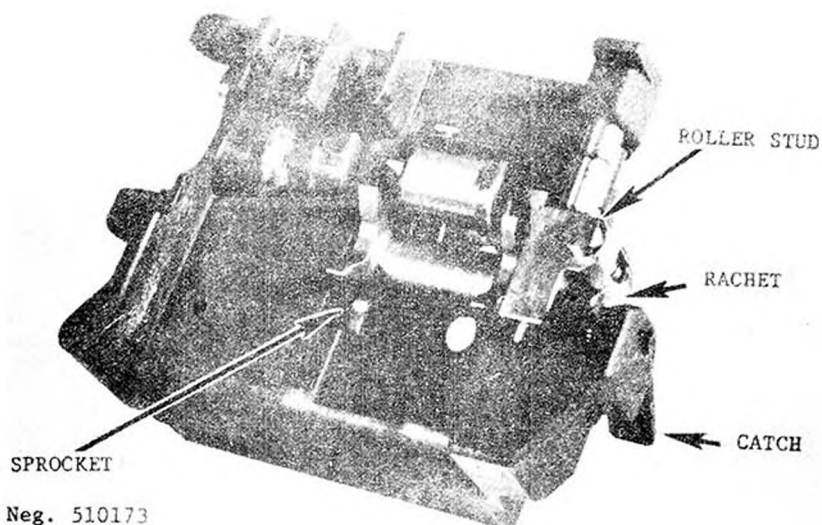
Figure 174. HK 21A1 feeder mechanism.
