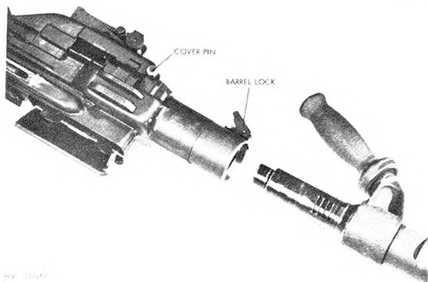
Figure 161. AA-52 barrel change.
