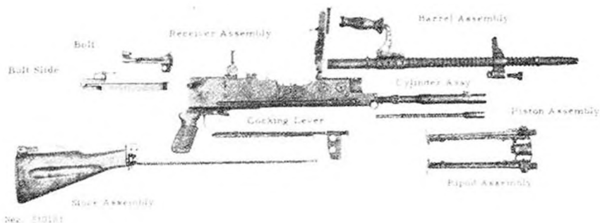
Figure 184. Type 62 disassembled.
