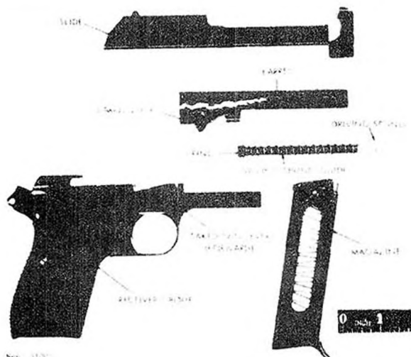
Figure 12. Beretta Model 1951 disassembled.
