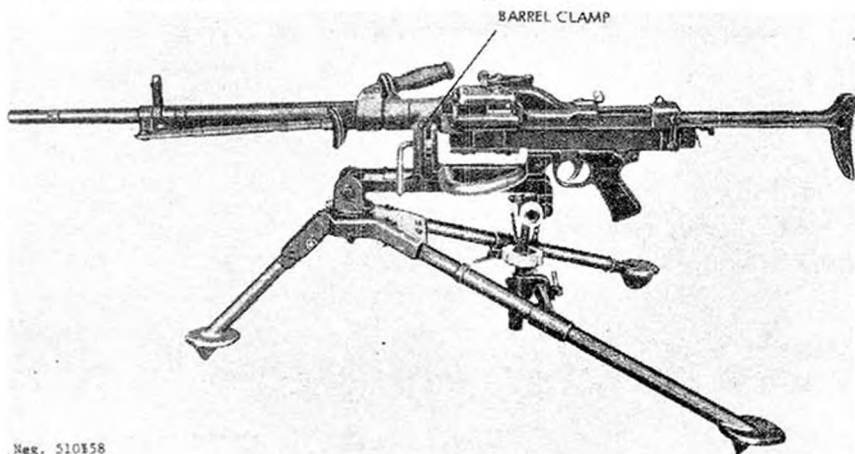
Figure 159. AA-52 heavy machinegun on tripod.
