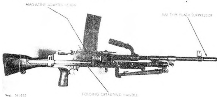
Figure 153. L4A1 Bren.
