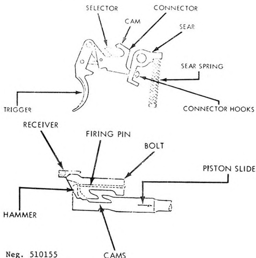
Figure 156. Bren bolt and trigger mechanism functioning.
