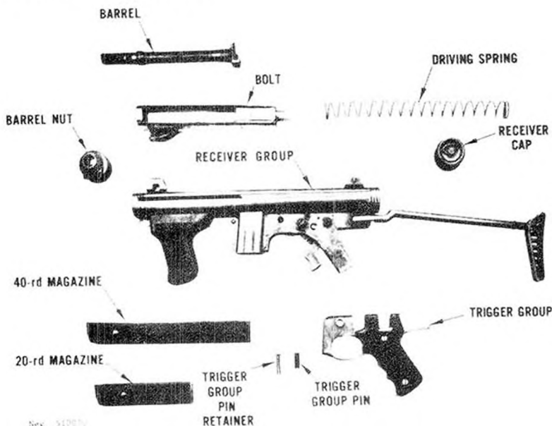
Figure 51. Beretta Model 12 disassembled.
