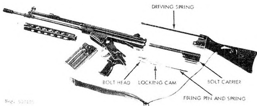
Figure 106. G3 disassembled.
