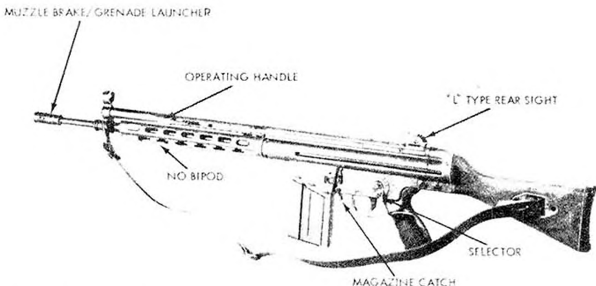
Figure 104. Early G3 (CETME) rifle.
