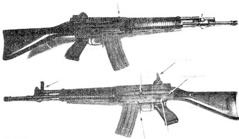
Figure 97. Italian Beretta M70/.223 rifle.
