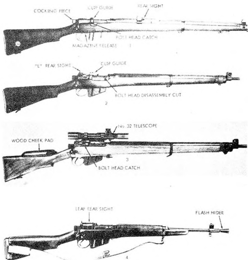
Figure 140. Lee Enfield rifles.
