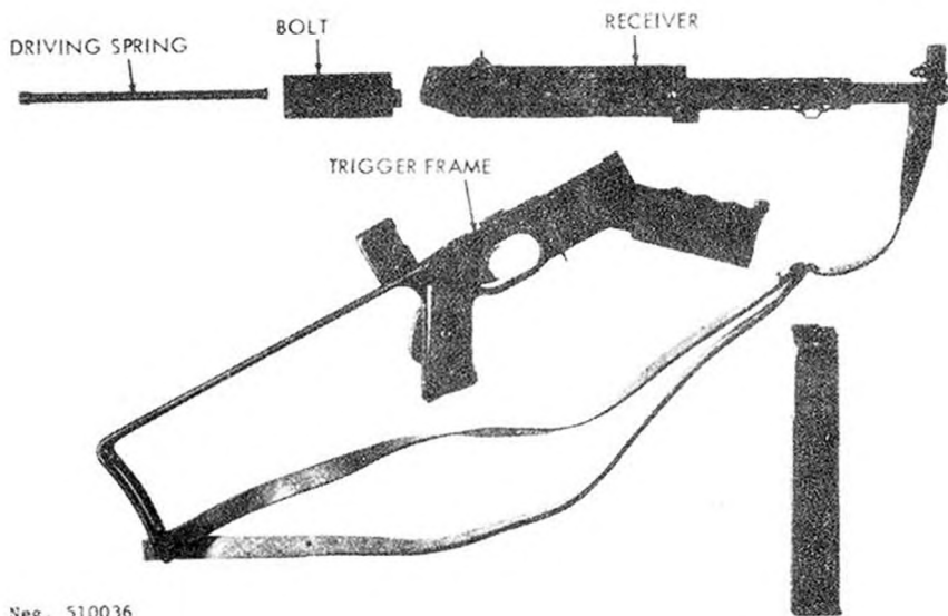
Figure 37. M.A.T. 49 disassembled.
