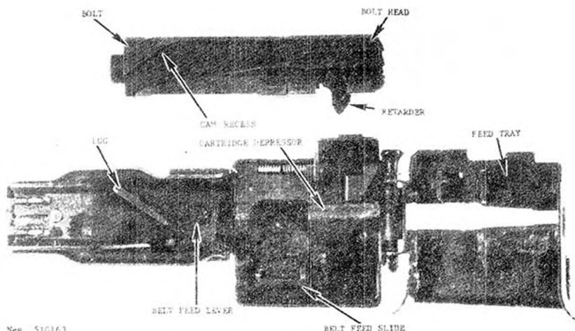
Figure 164. AA-52 bolt and feed cover.
