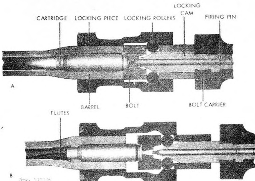
Figure 107. G3 bolt functioning.
