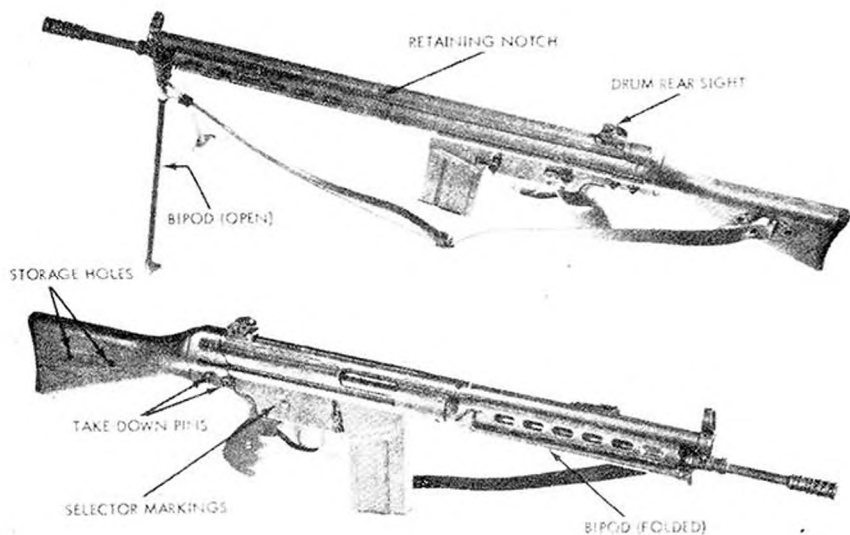
Figure 105. West German G3 rifle.
