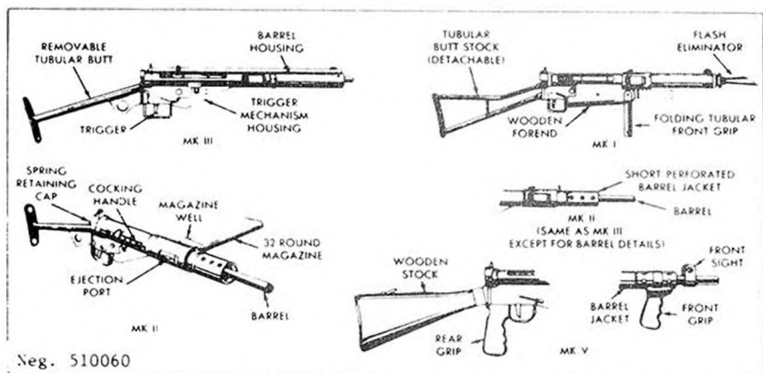
Figure 61. Sten Mark 1, 2, 3 and 5 submachineguns.
