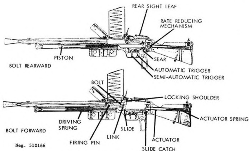
Figure 167. M24/29 section.
