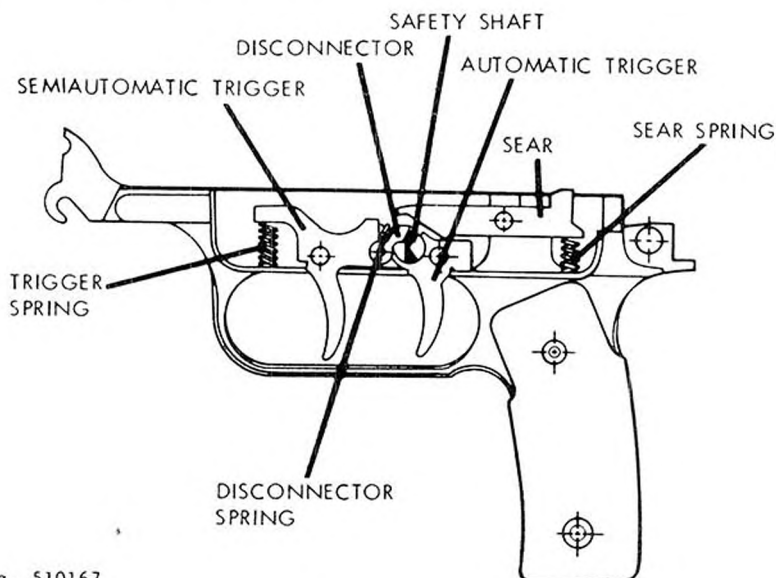
Figure 168. M24/29 trigger mechanism.
