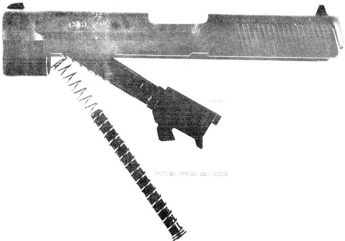
Neg. 529267 Figure 28.1.3. Removal of driving spring and barrel from Model 75 pistol.
