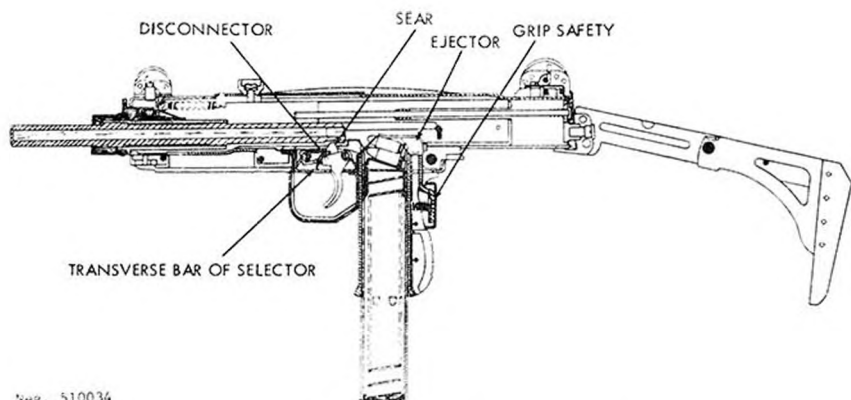
Figure 35. UZI submachinegun, section.
