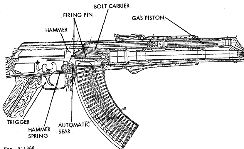
Figure 69. AK-47 section.
