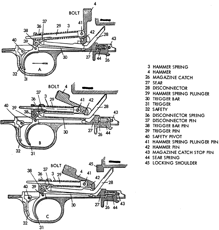
Figure 105. SKS trigger mechanism.
