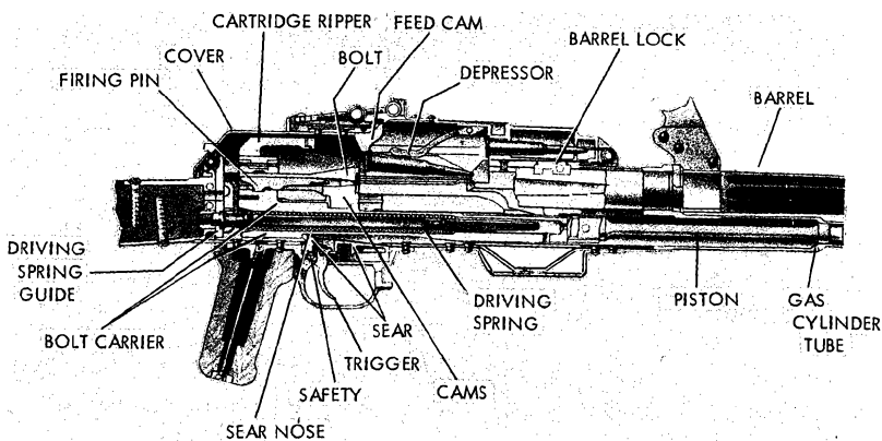
Figure 180. PK section.
