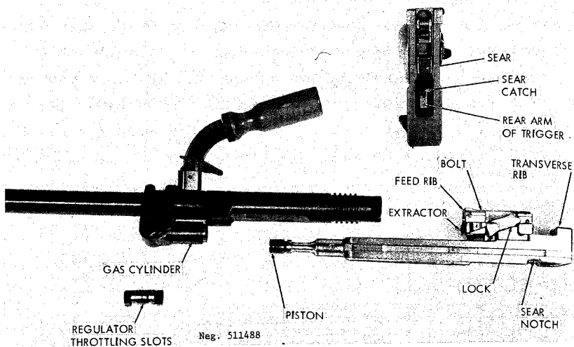
Figure 189. Vz59 mechanism.
