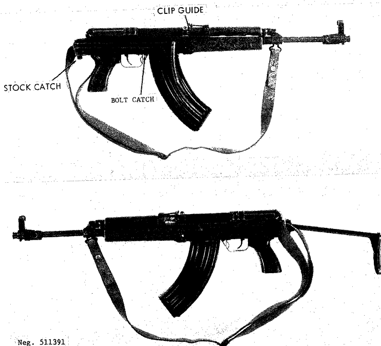
Figure 92. Czechoslovak M58V assault rifle.
