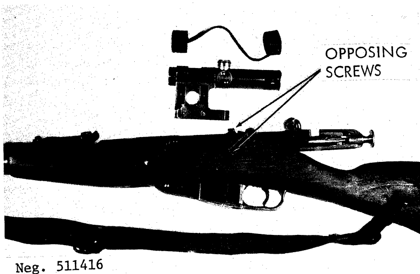
Figure 117. Zero adjustment for PU telescope.
