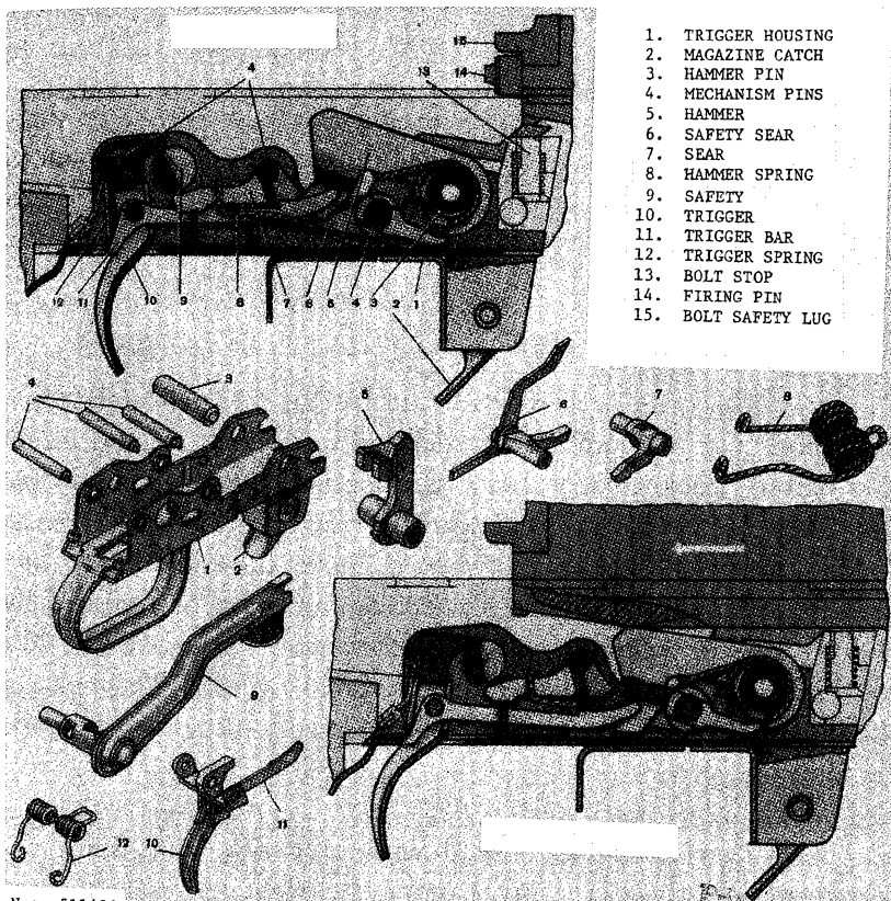
Figure 123. SVD trigger mechanism section.
