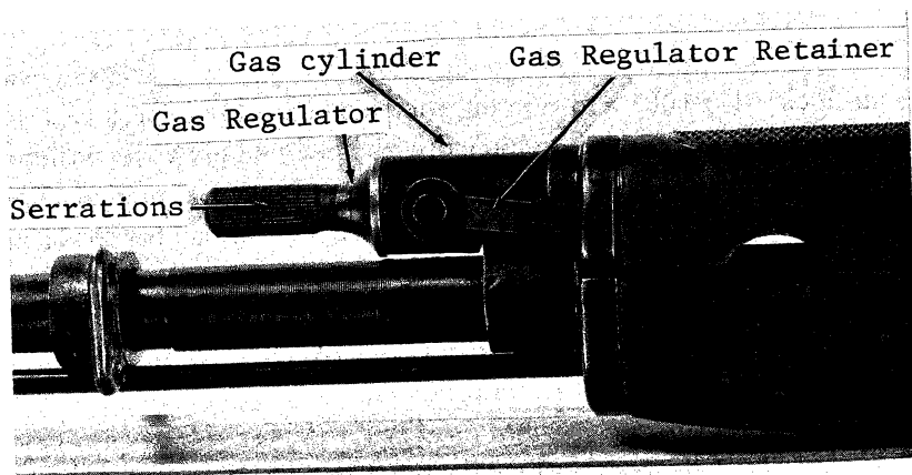
Figure 110. Gas regulator.
