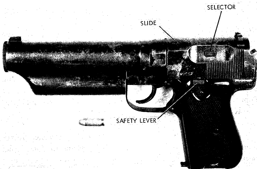
Figure 30. PRC Type 64 silenced pistol.
