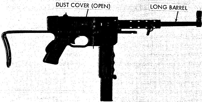
Figure 52. North Vietnamese modified M.A.T. 1949 submachinegun.
