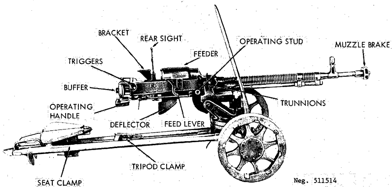
Figure 215. 12.7-mm DShK-38 heavy machinegun.
