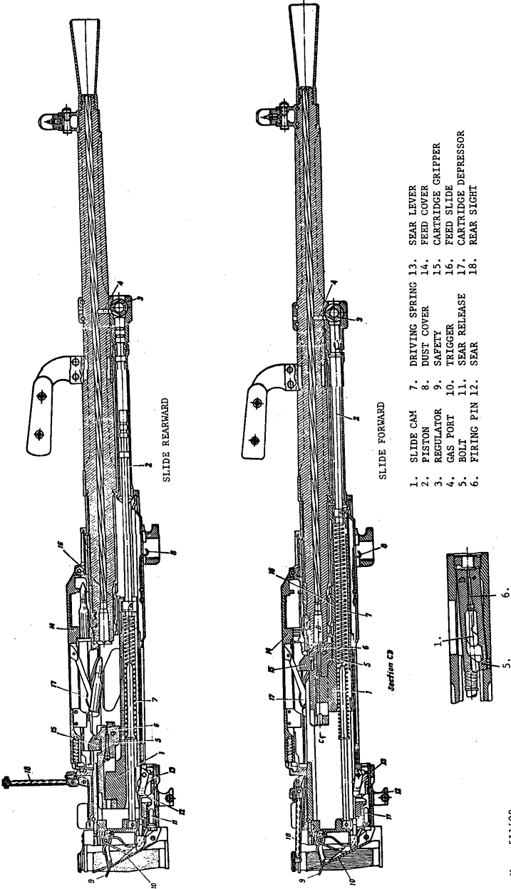
Figure 200. SGM section.
