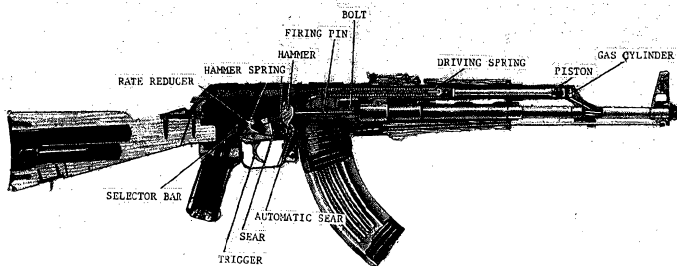
Figure 88. AKM section.
