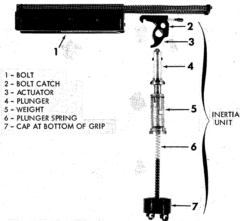
Figure 27. Vz61 rate reducer.
