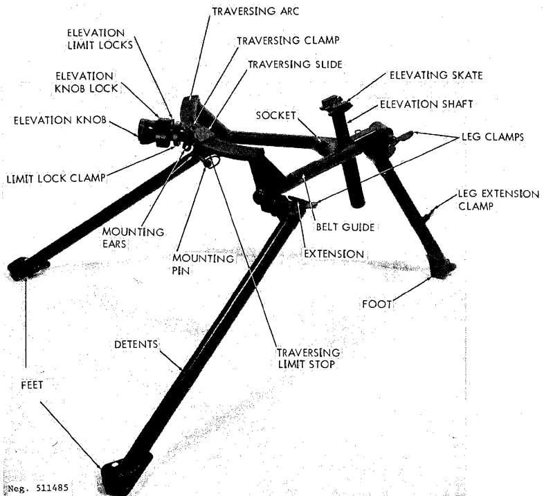
Figure 186. Vz59 tripod.
