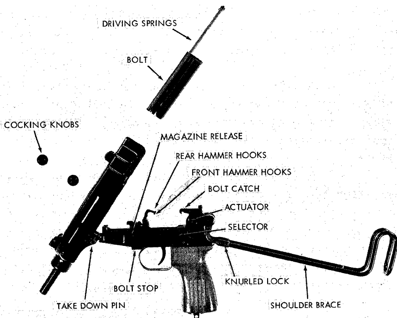
Figure 26. Vz61 disassembled.
