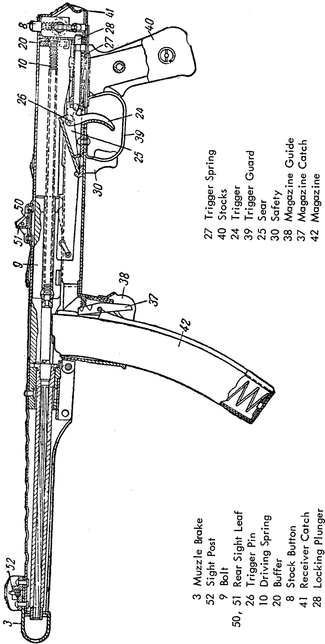
Figure 41. PPS-43 section.
