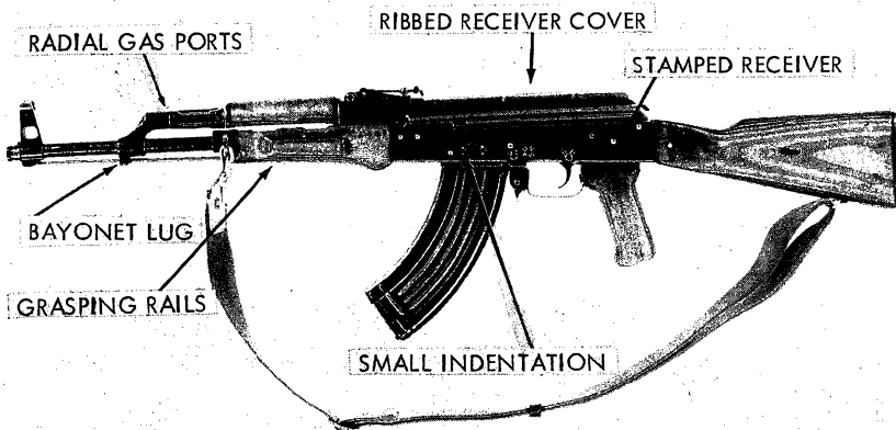
Figure 80. Soviet AKM assault rifle.
