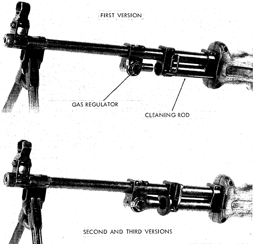
Figure 147. First and second model RPD gas cylinders.
