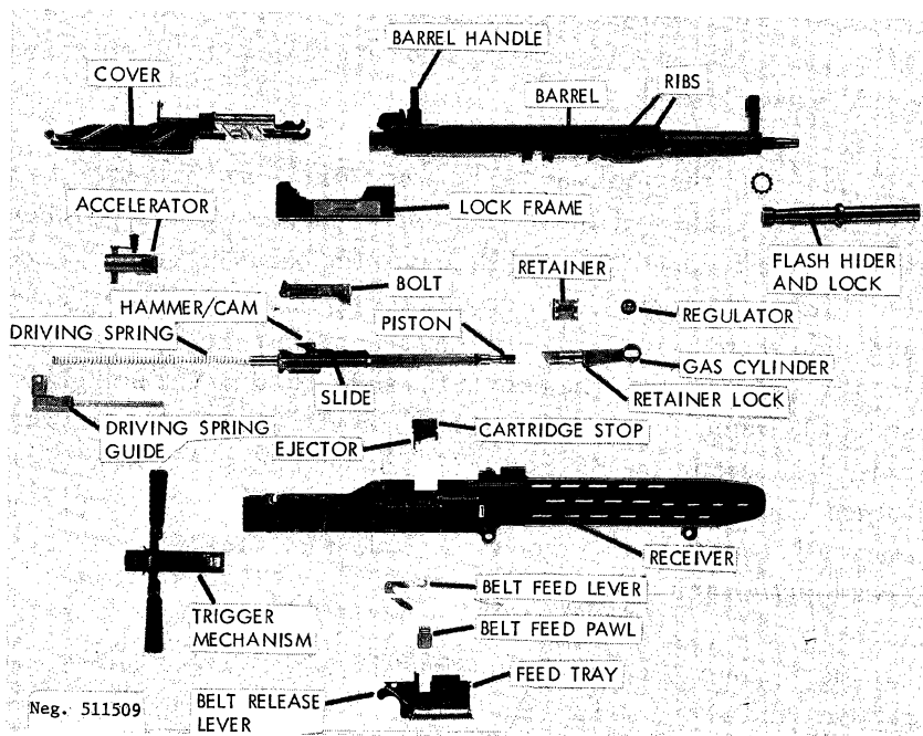
Figure 210. ZB-37 disassembled.
