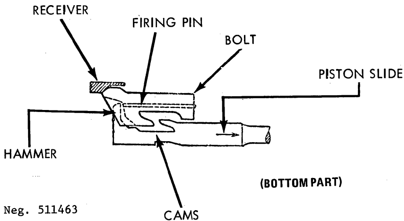
Figure 164. ZB30 bolt and trigger mechanism functioning.
