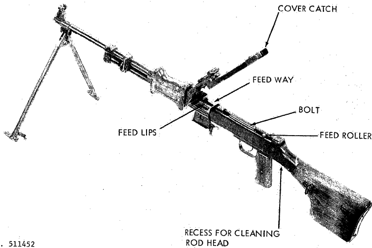
Figure 153. RPD ready for loading.
