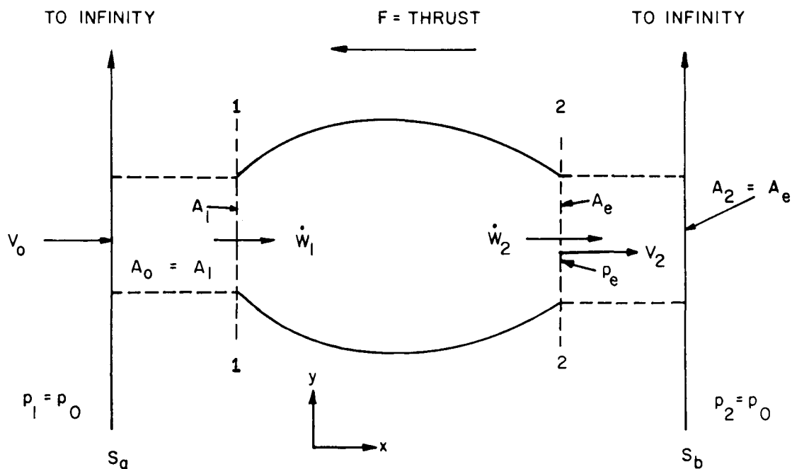
Figure 3-2. Application of the Momentum Theorem of Fluid Mechanics to an Arbitrary Propulsion System
