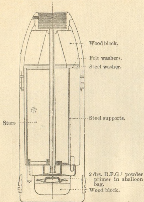
SHELL, Q.F. STAR, 4·5-INCH HOWITZER.
